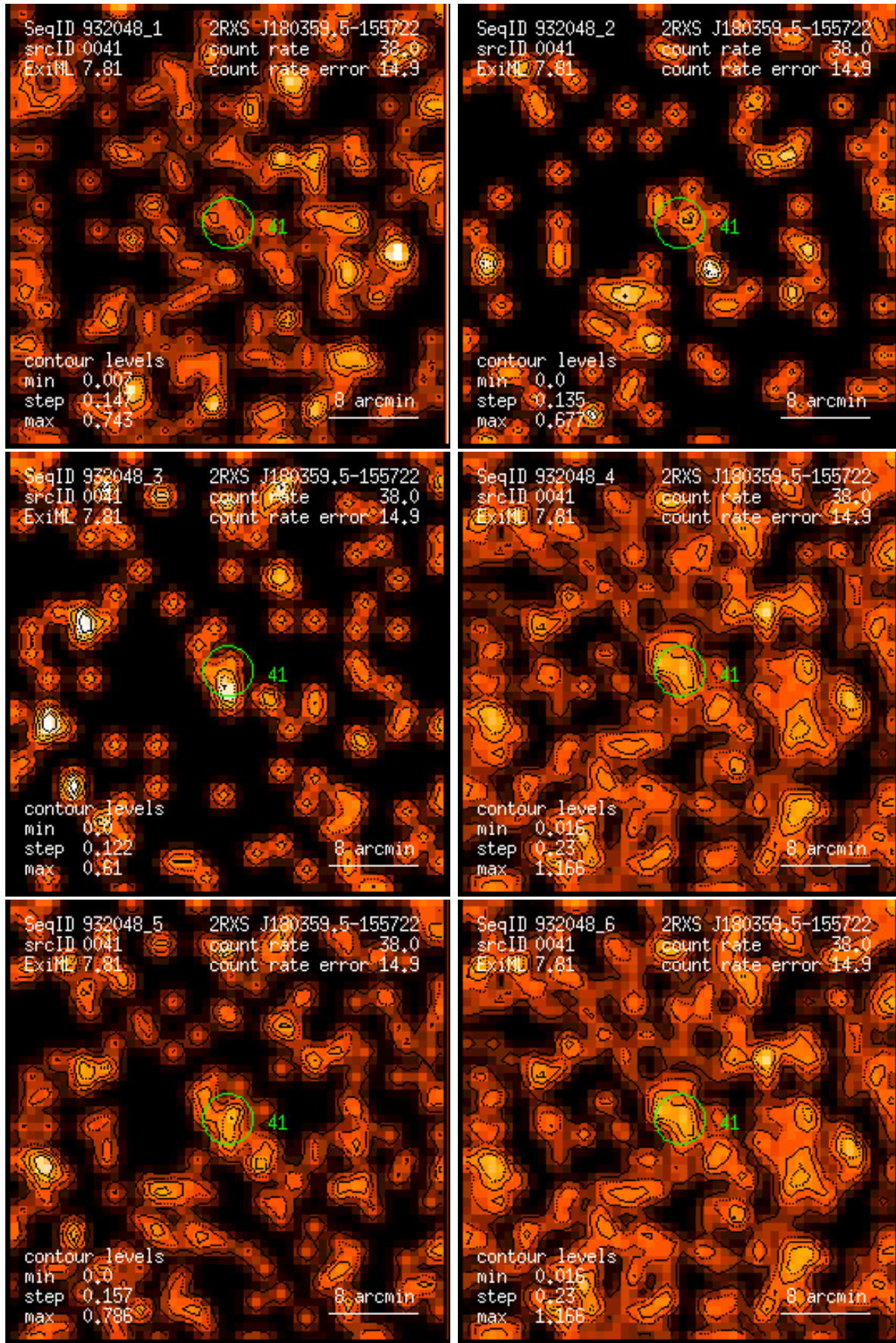
Figure 41: RASS 932048: detection 0041: band rate images, Gaussian filter: (1) PSPC channels 11 – 41, (2) 52 – 90, (3) 91 – 201, (4) 11 – 235, (5) 52 – 201, (6) 11 – 201. Broad band rates in counts/ks. Band rate contour levels in counts/ks/arcmin 2 .
