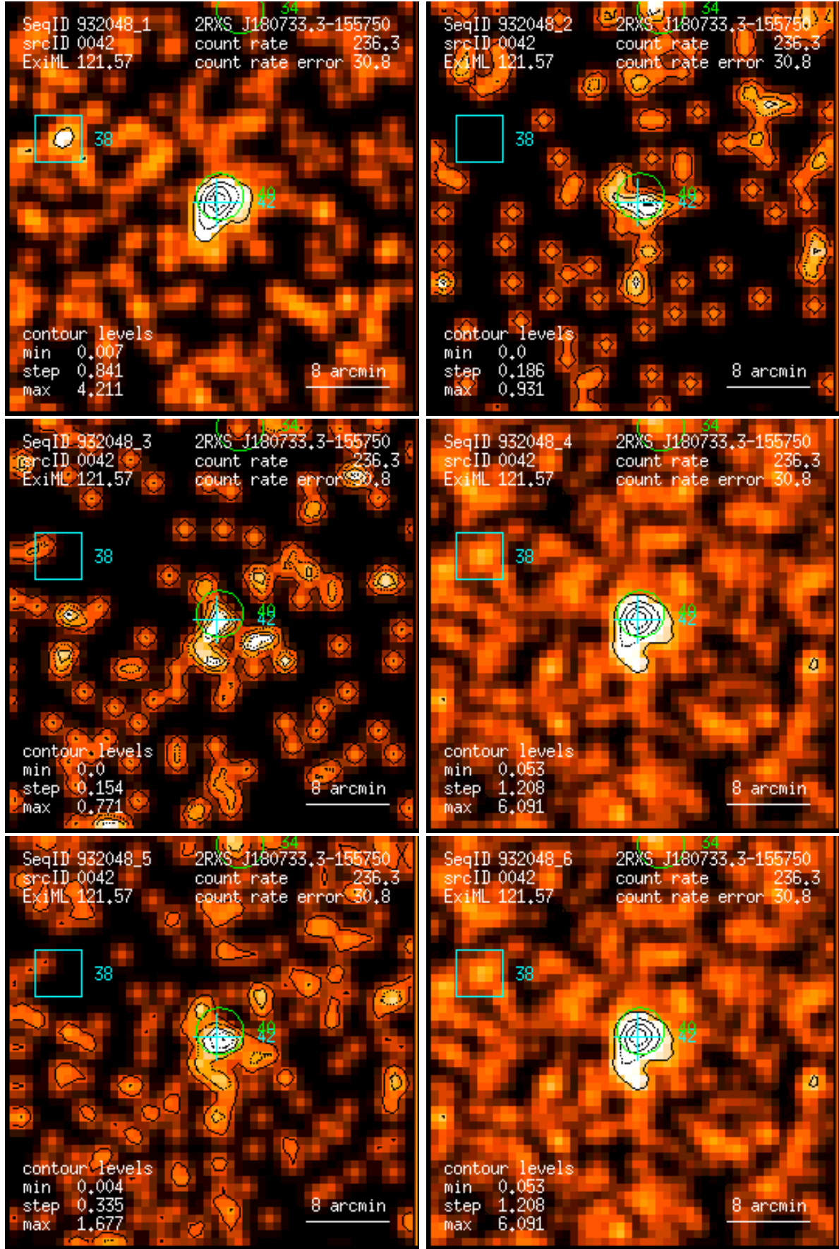
Figure 42: RASS 932048: detection 0042: band rate images, Gaussian filter: (1) PSPC channels 11 – 41, (2) 52 – 90, (3) 91 – 201, (4) 11 – 235, (5) 52 – 201, (6) 11 – 201. Broad band rates in counts/ks. Band rate contour levels in counts/ks/arcmin 2 .
