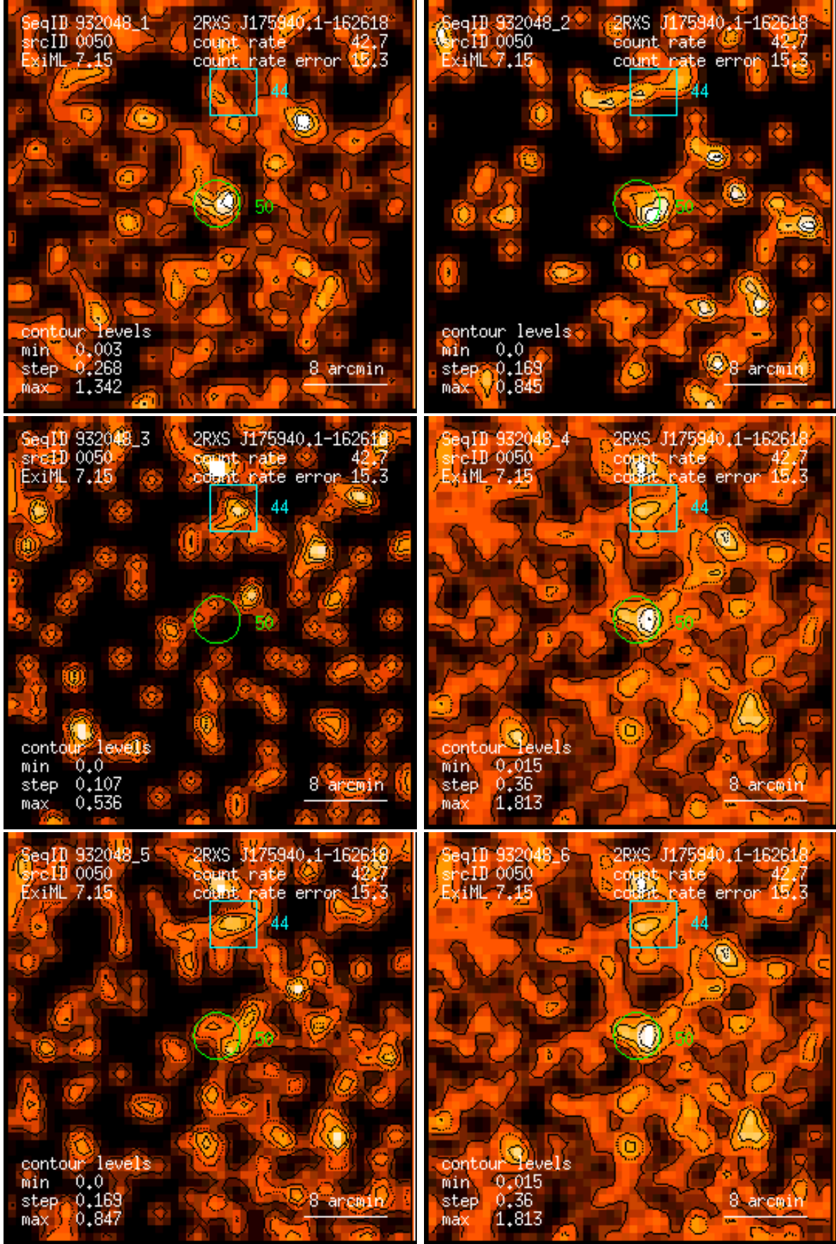
Figure 50: RASS 932048: detection 0050: band rate images, Gaussian filter: (1) PSPC channels 11 – 41, (2) 52 – 90, (3) 91 – 201, (4) 11 – 235, (5) 52 – 201, (6) 11 – 201. Broad band rates in counts/ks. Band rate contour levels in counts/ks/arcmin 2 .
