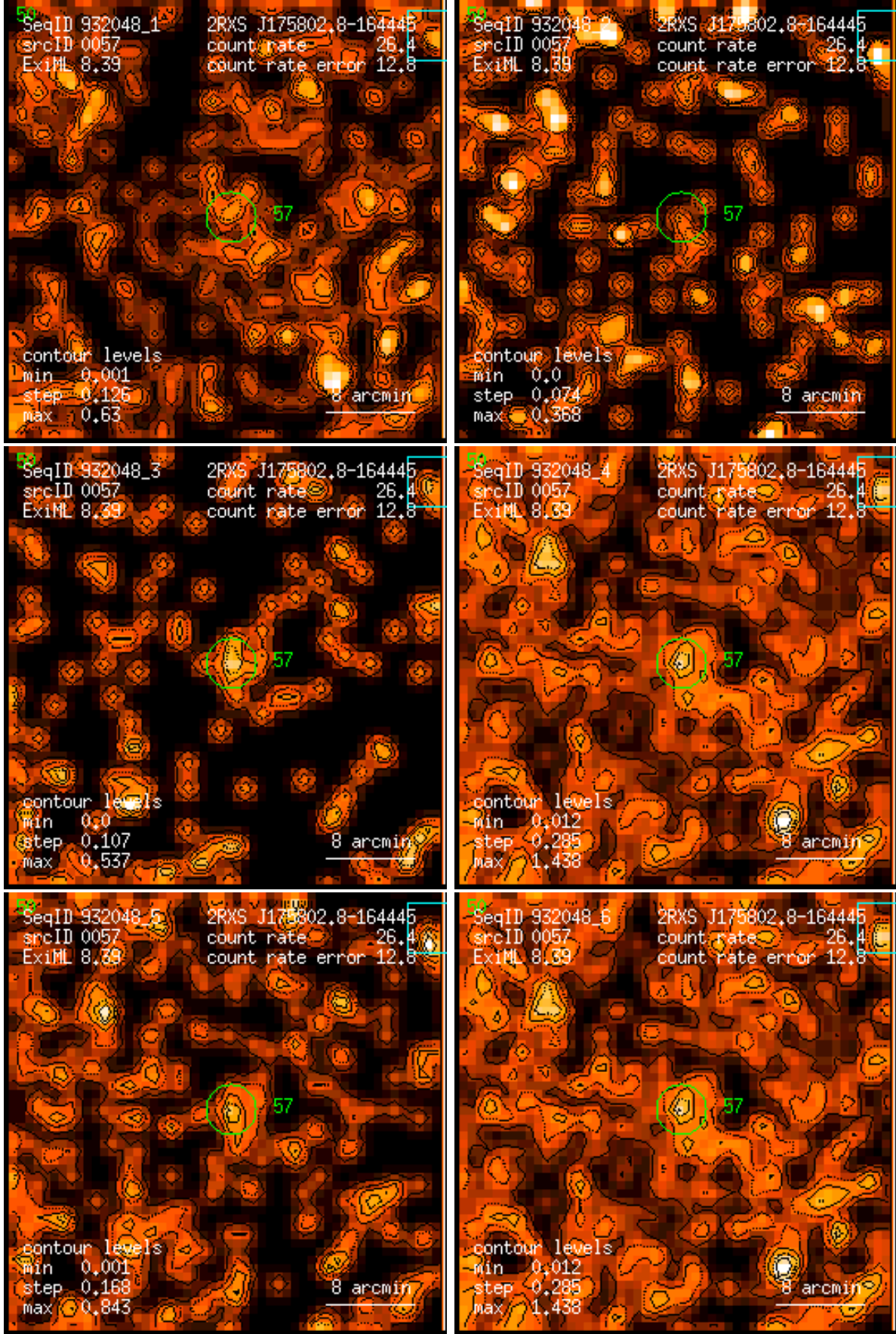
Figure 57: RASS 932048: detection 0057: band rate images, Gaussian filter: (1) PSPC channels 11 – 41, (2) 52 – 90, (3) 91 – 201, (4) 11 – 235, (5) 52 – 201, (6) 11 – 201. Broad band rates in counts/ks. Band rate contour levels in counts/ks/arcmin 2 .
