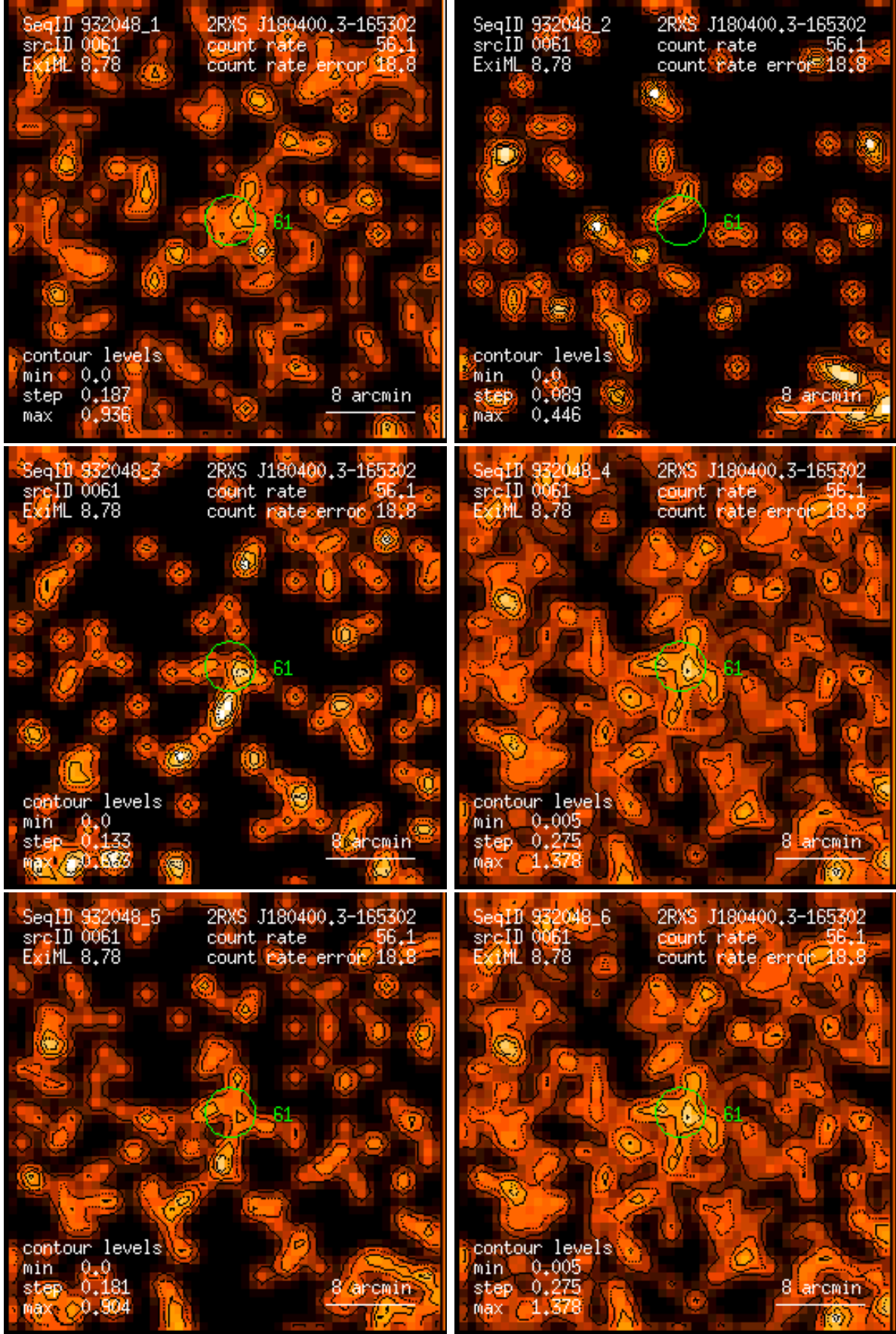
Figure 61: RASS 932048: detection 0061: band rate images, Gaussian filter: (1) PSPC channels 11 – 41, (2) 52 – 90, (3) 91 – 201, (4) 11 – 235, (5) 52 – 201, (6) 11 – 201. Broad band rates in counts/ks. Band rate contour levels in counts/ks/arcmin 2 .
