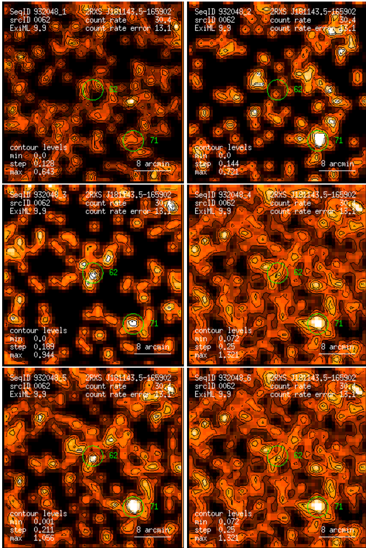
Figure 62: RASS 932048: detection 0062: band rate images, Gaussian filter: (1) PSPC channels 11 – 41, (2) 52 – 90, (3) 91 – 201, (4) 11 – 235, (5) 52 – 201, (6) 11 – 201. Broad band rates in counts/ks. Band rate contour levels in counts/ks/arcmin 2 .
