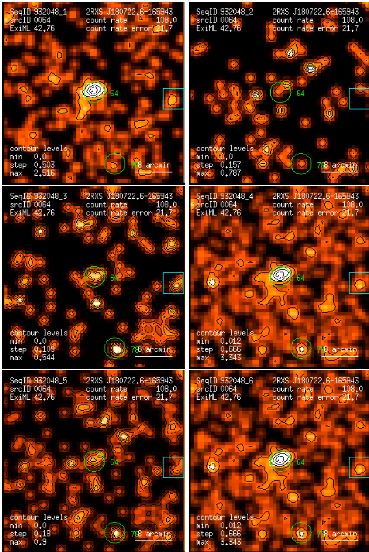
Figure 64: RASS 932048: detection 0064: band rate images, Gaussian filter: (1) PSPC channels 11 – 41, (2) 52 – 90, (3) 91 – 201, (4) 11 – 235, (5) 52 – 201, (6) 11 – 201. Broad band rates in counts/ks. Band rate contour levels in counts/ks/arcmin 2 .
