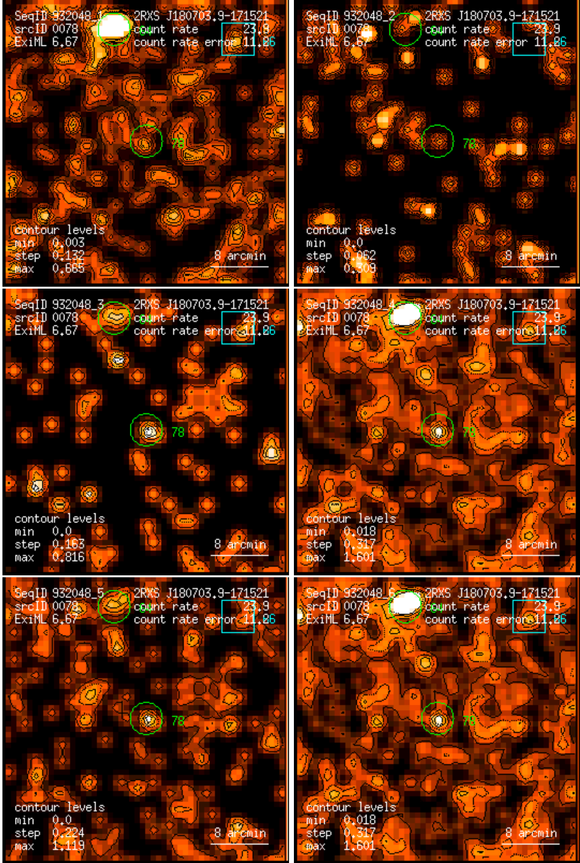
Figure 78: RASS 932048: detection 0078: band rate images, Gaussian filter: (1) PSPC channels 11 – 41, (2) 52 – 90, (3) 91 – 201, (4) 11 – 235, (5) 52 – 201, (6) 11 – 201. Broad band rates in counts/ks. Band rate contour levels in counts/ks/arcmin 2 .
