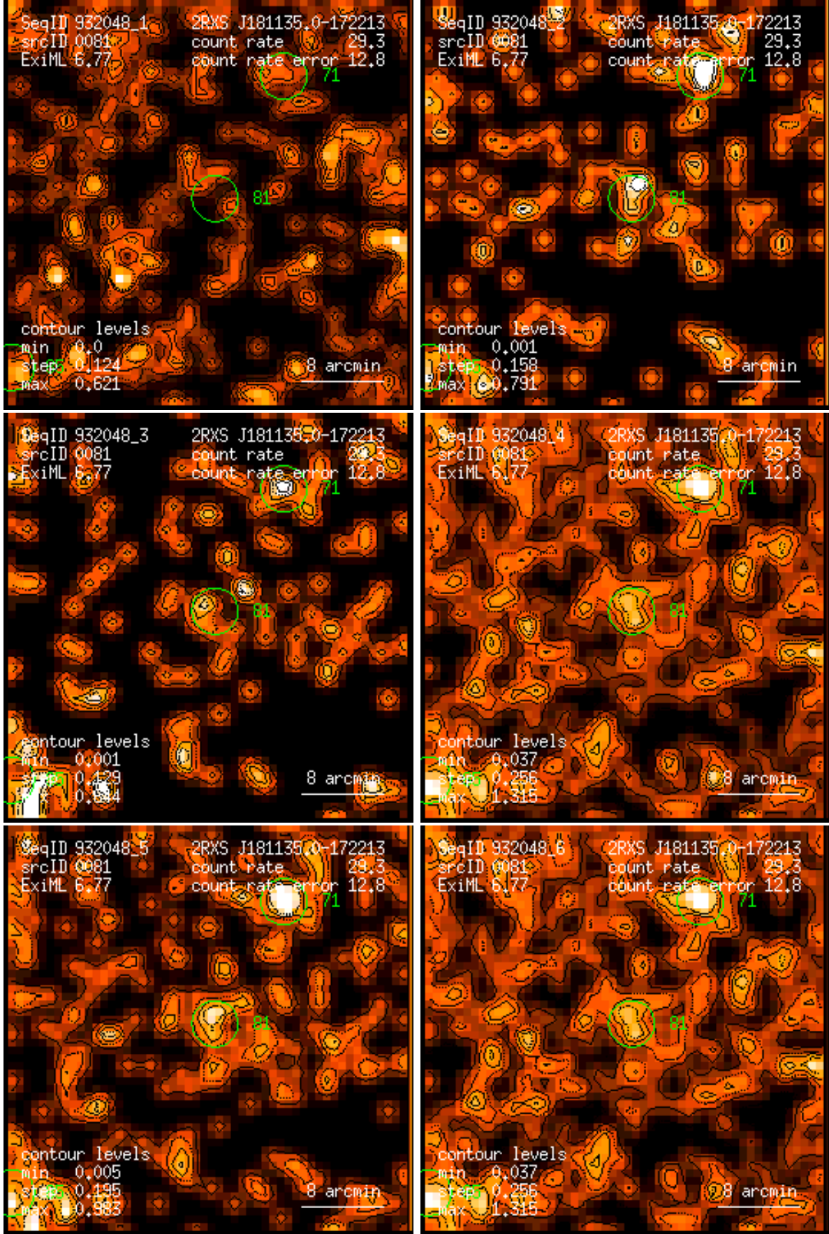
Figure 81: RASS 932048: detection 0081: band rate images, Gaussian filter: (1) PSPC channels 11 – 41, (2) 52 – 90, (3) 91 – 201, (4) 11 – 235, (5) 52 – 201, (6) 11 – 201. Broad band rates in counts/ks. Band rate contour levels in counts/ks/arcmin 2 .
