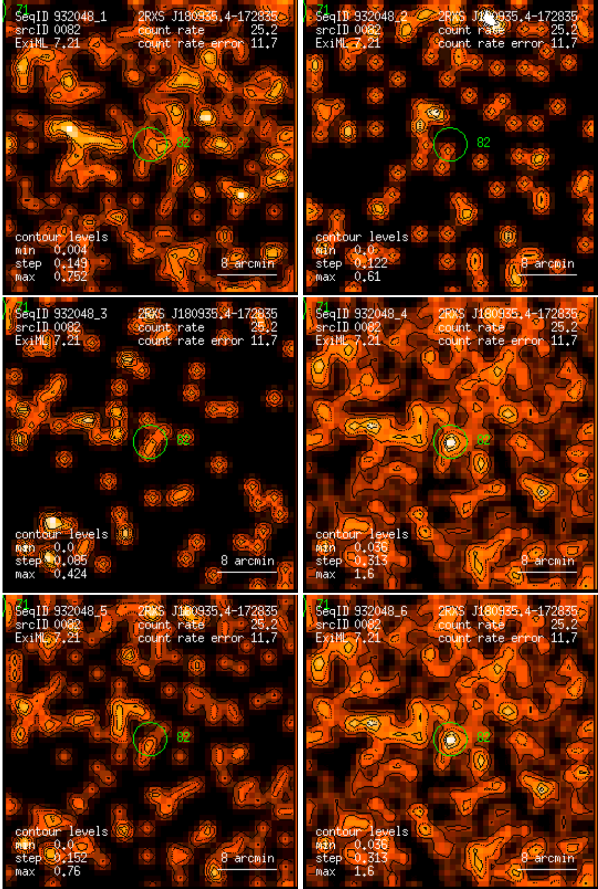
Figure 82: RASS 932048: detection 0082: band rate images, Gaussian filter: (1) PSPC channels 11 – 41, (2) 52 – 90, (3) 91 – 201, (4) 11 – 235, (5) 52 – 201, (6) 11 – 201. Broad band rates in counts/ks. Band rate contour levels in counts/ks/arcmin 2 .
