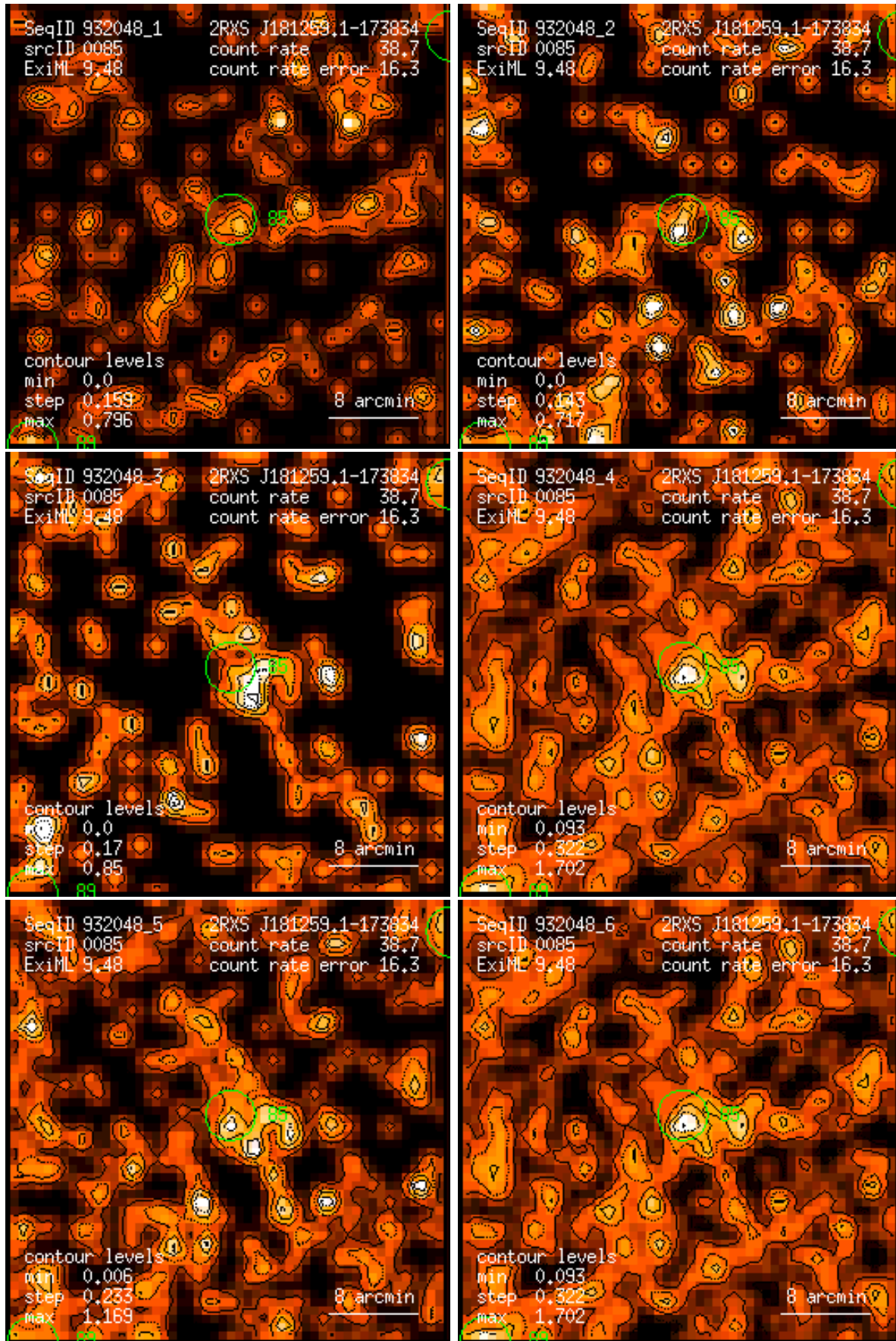
Figure 85: RASS 932048: detection 0085: band rate images, Gaussian filter: (1) PSPC channels 11 – 41, (2) 52 – 90, (3) 91 – 201, (4) 11 – 235, (5) 52 – 201, (6) 11 – 201. Broad band rates in counts/ks. Band rate contour levels in counts/ks/arcmin 2 .
