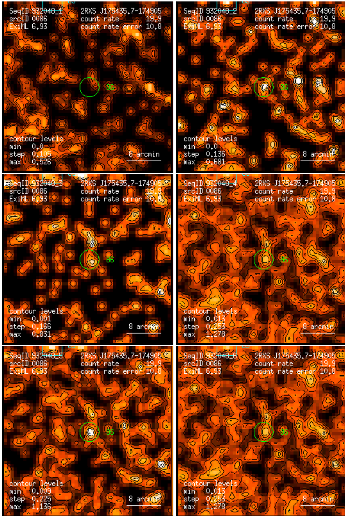
Figure 86: RASS 932048: detection 0086: band rate images, Gaussian filter: (1) PSPC channels 11 – 41, (2) 52 – 90, (3) 91 – 201, (4) 11 – 235, (5) 52 – 201, (6) 11 – 201. Broad band rates in counts/ks. Band rate contour levels in counts/ks/arcmin 2 .
