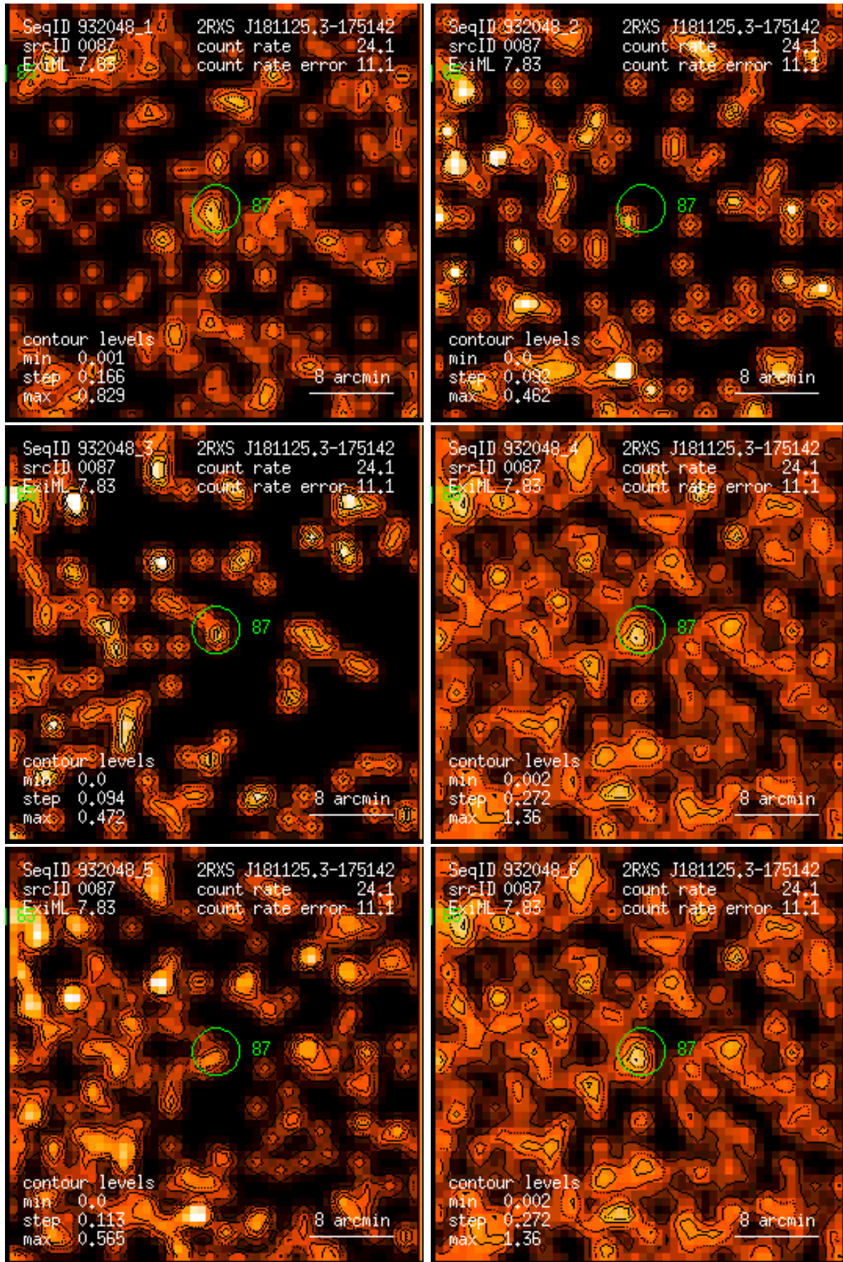
Figure 87: RASS 932048: detection 0087: band rate images, Gaussian filter: (1) PSPC channels 11 – 41, (2) 52 – 90, (3) 91 – 201, (4) 11 – 235, (5) 52 – 201, (6) 11 – 201. Broad band rates in counts/ks. Band rate contour levels in counts/ks/arcmin 2 .
