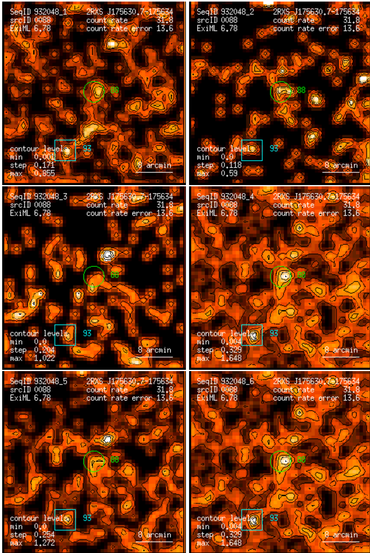
Figure 88: RASS 932048: detection 0088: band rate images, Gaussian filter: (1) PSPC channels 11 – 41, (2) 52 – 90, (3) 91 – 201, (4) 11 – 235, (5) 52 – 201, (6) 11 – 201. Broad band rates in counts/ks. Band rate contour levels in counts/ks/arcmin 2 .
