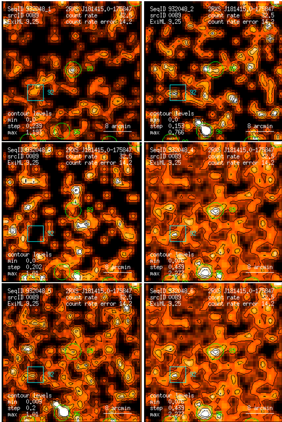
Figure 89: RASS 932048: detection 0089: band rate images, Gaussian filter: (1) PSPC channels 11 – 41, (2) 52 – 90, (3) 91 – 201, (4) 11 – 235, (5) 52 – 201, (6) 11 – 201. Broad band rates in counts/ks. Band rate contour levels in counts/ks/arcmin 2 .
