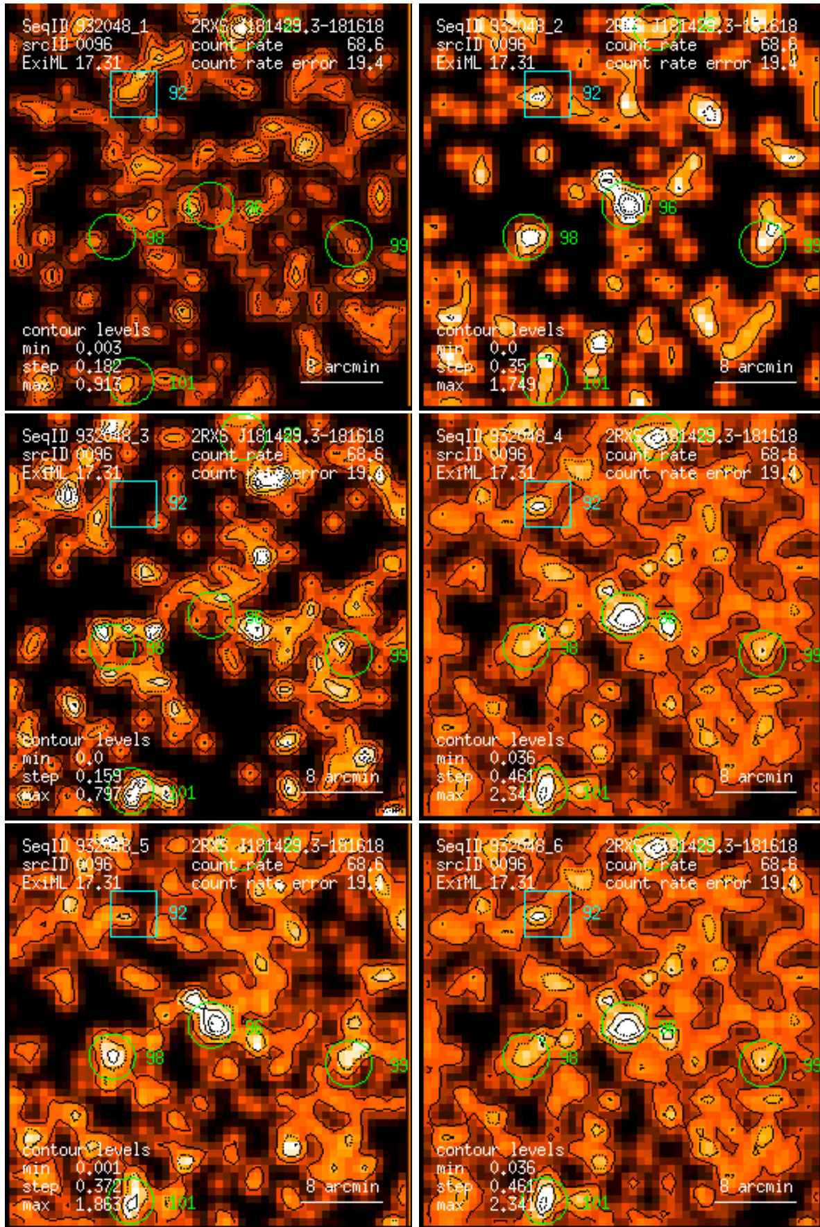
Figure 96: RASS 932048: detection 0096: band rate images, Gaussian filter: (1) PSPC channels 11 – 41, (2) 52 – 90, (3) 91 – 201, (4) 11 – 235, (5) 52 – 201, (6) 11 – 201. Broad band rates in counts/ks. Band rate contour levels in counts/ks/arcmin 2 .
