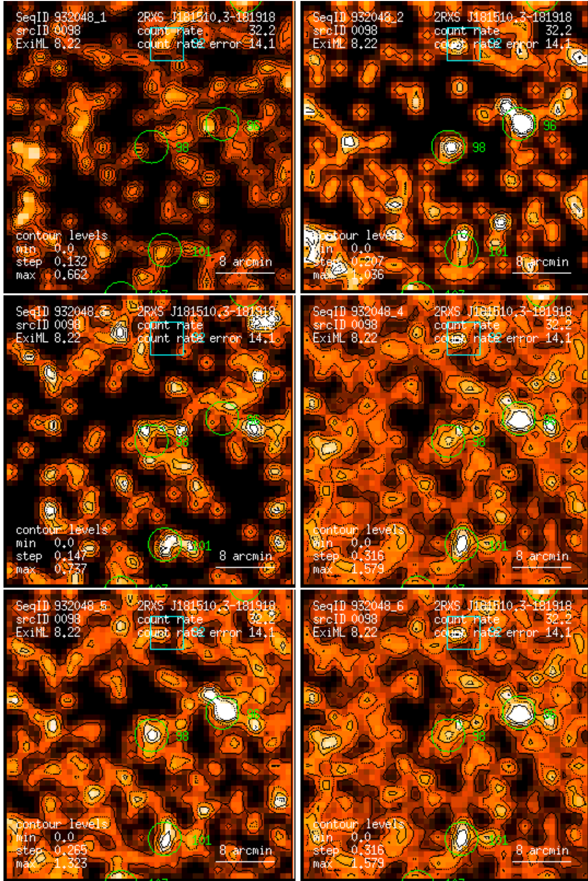
Figure 98: RASS 932048: detection 0098: band rate images, Gaussian filter: (1) PSPC channels 11 – 41, (2) 52 – 90, (3) 91 – 201, (4) 11 – 235, (5) 52 – 201, (6) 11 – 201. Broad band rates in counts/ks. Band rate contour levels in counts/ks/arcmin 2 .
