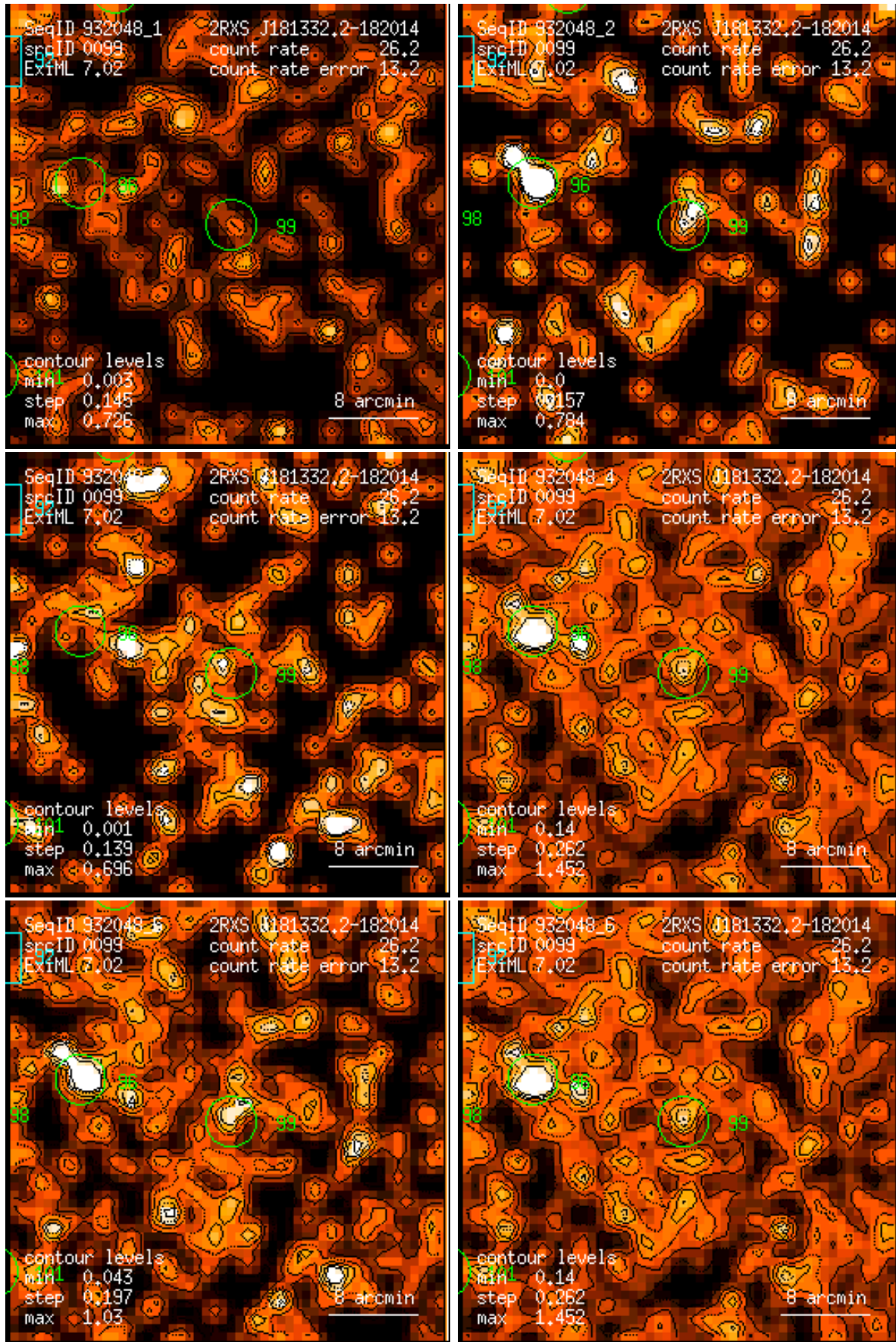
Figure 99: RASS 932048: detection 0099: band rate images, Gaussian filter: (1) PSPC channels 11 – 41, (2) 52 – 90, (3) 91 – 201, (4) 11 – 235, (5) 52 – 201, (6) 11 – 201. Broad band rates in counts/ks. Band rate contour levels in counts/ks/arcmin 2 .
