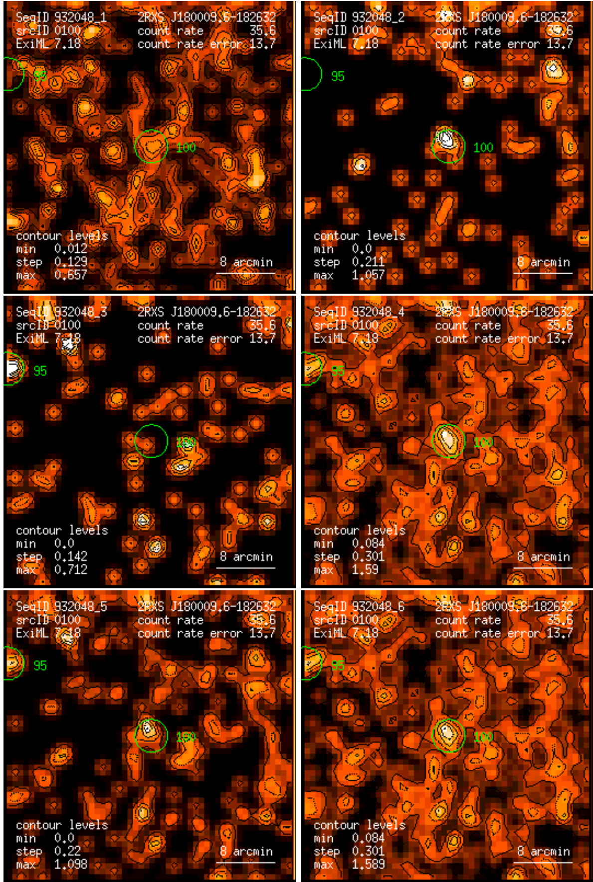
Figure 100: RASS 932048: detection 0100: band rate images, Gaussian filter: (1) PSPC channels 11 – 41, (2) 52 – 90, (3) 91 – 201, (4) 11 – 235, (5) 52 – 201, (6) 11 – 201. Broad band rates in counts/ks. Band rate contour levels in counts/ks/arcmin 2 .
