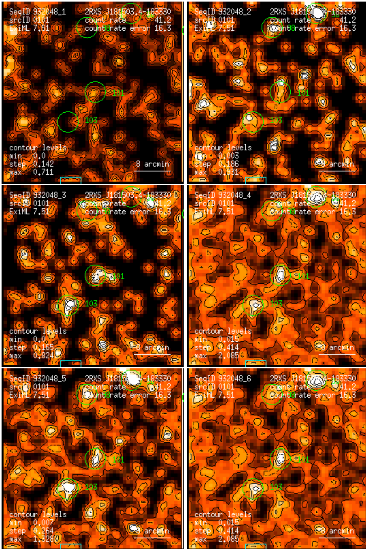
Figure 101: RASS 932048: detection 0101: band rate images, Gaussian filter: (1) PSPC channels 11 – 41, (2) 52 – 90, (3) 91 – 201, (4) 11 – 235, (5) 52 – 201, (6) 11 – 201. Broad band rates in counts/ks. Band rate contour levels in counts/ks/arcmin 2 .
