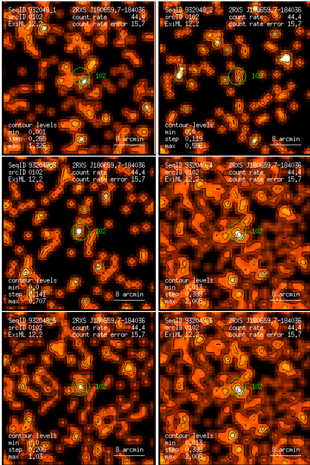
Figure 102: RASS 932048: detection 0102: band rate images, Gaussian filter: (1) PSPC channels 11 – 41, (2) 52 – 90, (3) 91 – 201, (4) 11 – 235, (5) 52 – 201, (6) 11 – 201. Broad band rates in counts/ks. Band rate contour levels in counts/ks/arcmin 2 .
