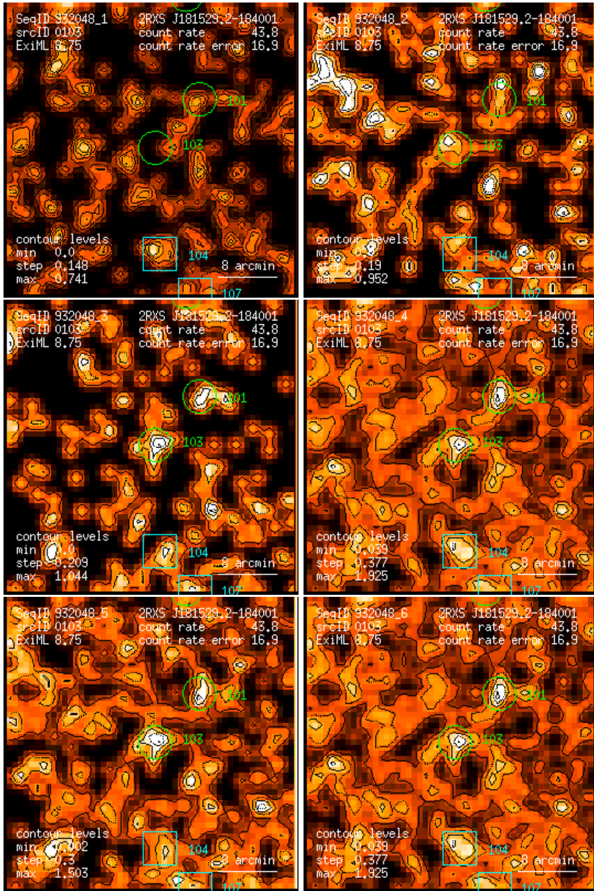
Figure 103: RASS 932048: detection 0103: band rate images, Gaussian filter: (1) PSPC channels 11 – 41, (2) 52 – 90, (3) 91 – 201, (4) 11 – 235, (5) 52 – 201, (6) 11 – 201. Broad band rates in counts/ks. Band rate contour levels in counts/ks/arcmin 2 .
