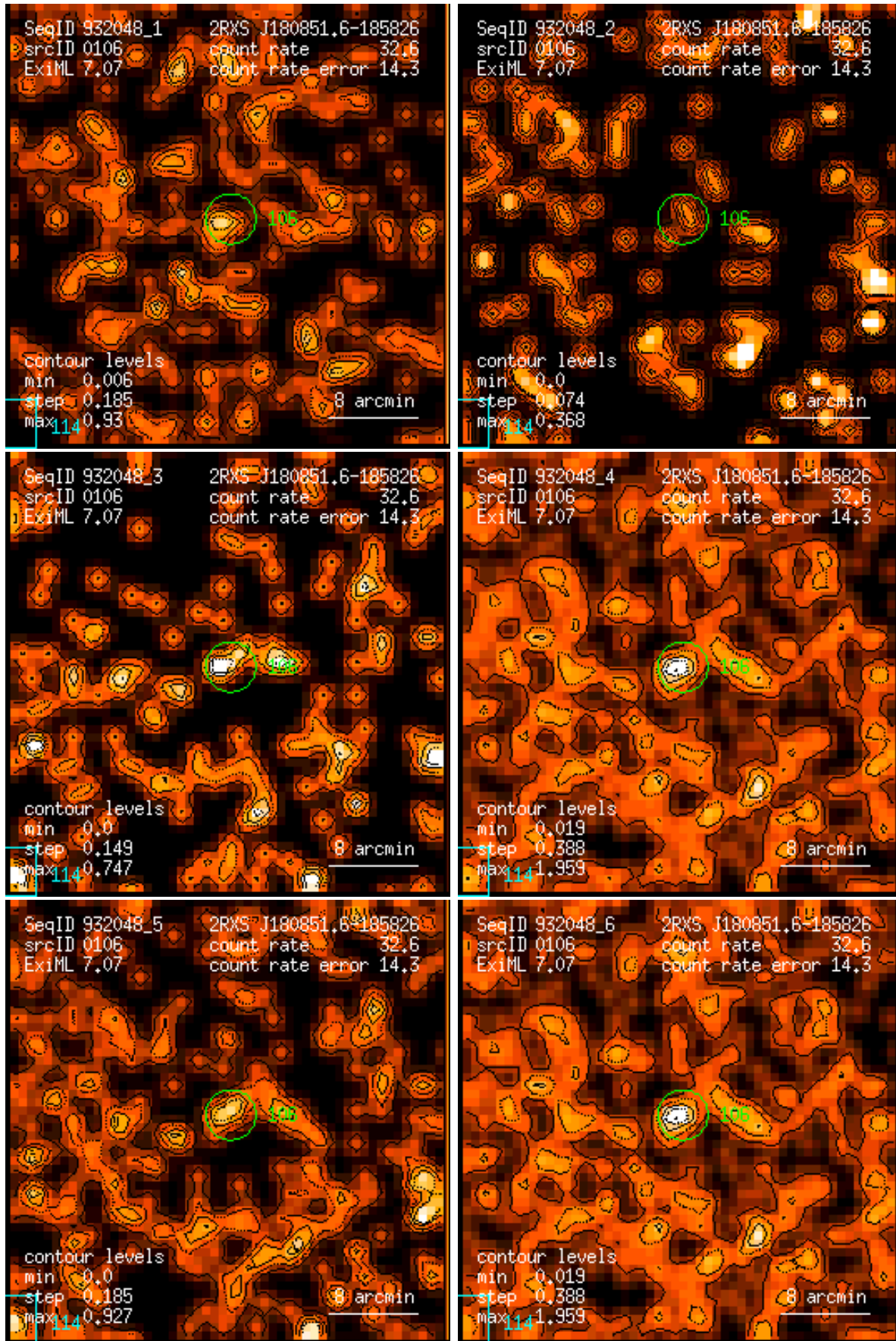
Figure 106: RASS 932048: detection 0106: band rate images, Gaussian filter: (1) PSPC channels 11 – 41, (2) 52 – 90, (3) 91 – 201, (4) 11 – 235, (5) 52 – 201, (6) 11 – 201. Broad band rates in counts/ks. Band rate contour levels in counts/ks/arcmin 2 .
