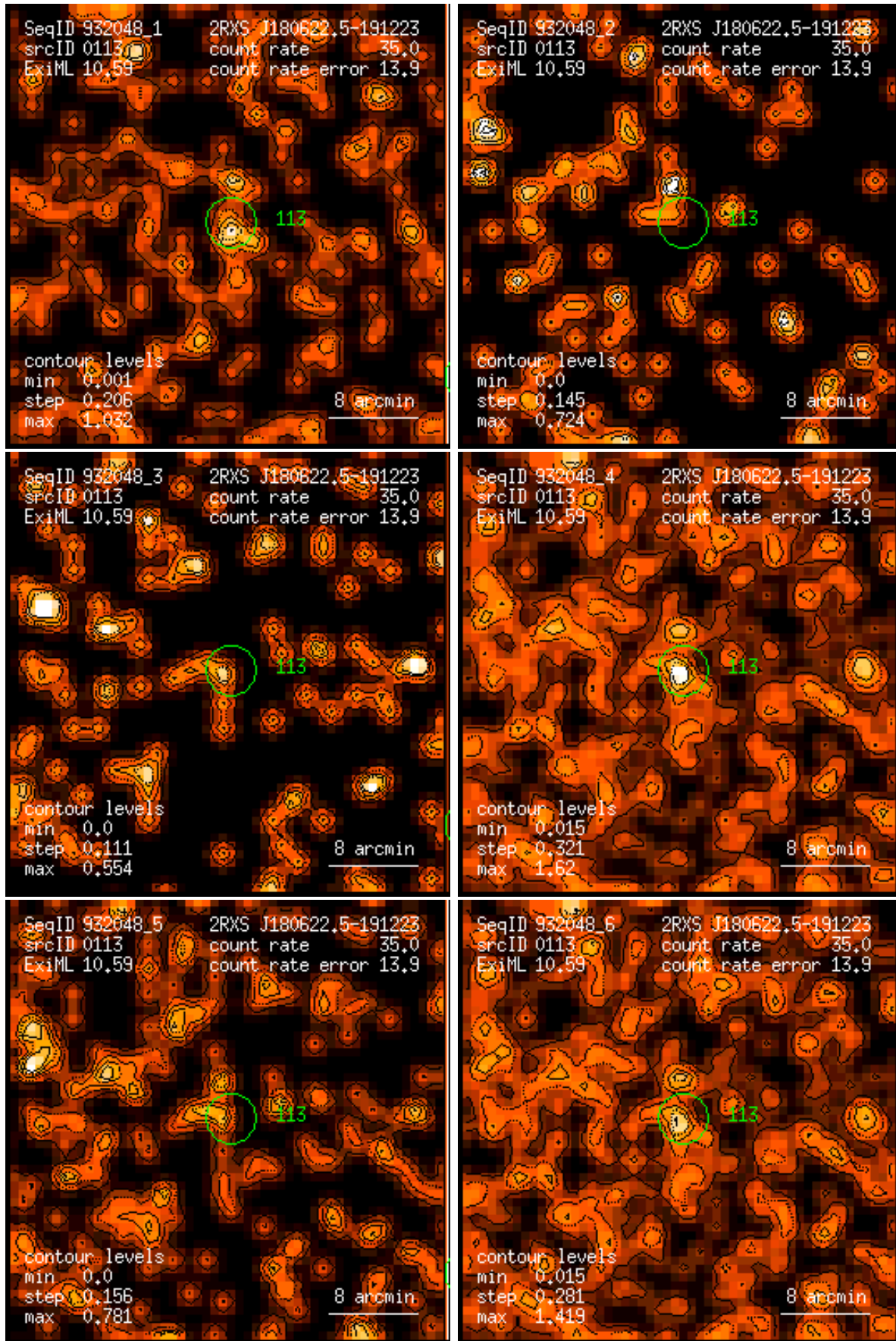
Figure 113: RASS 932048: detection 0113: band rate images, Gaussian filter: (1) PSPC channels 11 – 41, (2) 52 – 90, (3) 91 – 201, (4) 11 – 235, (5) 52 – 201, (6) 11 – 201. Broad band rates in counts/ks. Band rate contour levels in counts/ks/arcmin 2 .
