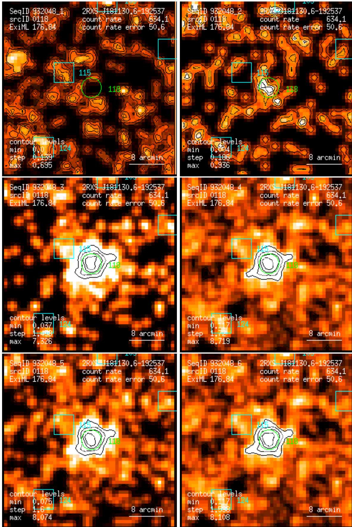
Figure 118: RASS 932048: detection 0118: band rate images, Gaussian filter: (1) PSPC channels 11 – 41, (2) 52 – 90, (3) 91 – 201, (4) 11 – 235, (5) 52 – 201, (6) 11 – 201. Broad band rates in counts/ks. Band rate contour levels in counts/ks/arcmin 2 .
