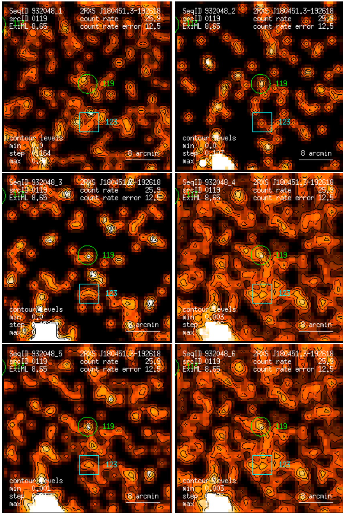
Figure 119: RASS 932048: detection 0119: band rate images, Gaussian filter: (1) PSPC channels 11 – 41, (2) 52 – 90, (3) 91 – 201, (4) 11 – 235, (5) 52 – 201, (6) 11 – 201. Broad band rates in counts/ks. Band rate contour levels in counts/ks/arcmin 2 .
