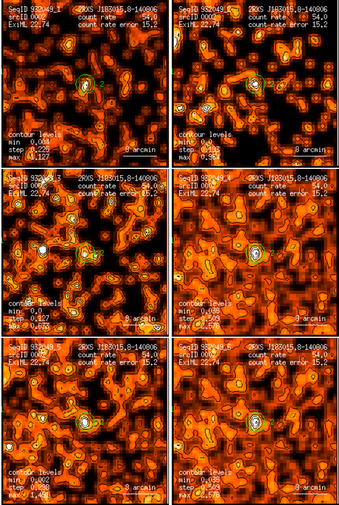
Figure 2: RASS 932049: detection 0002: band rate images, Gaussian filter: (1) PSPC channels 11 – 41, (2) 52 – 90, (3) 91 – 201, (4) 11 – 235, (5) 52 – 201, (6) 11 – 201. Broad band rates in counts/ks. Band rate contour levels in counts/ks/arcmin 2 .
