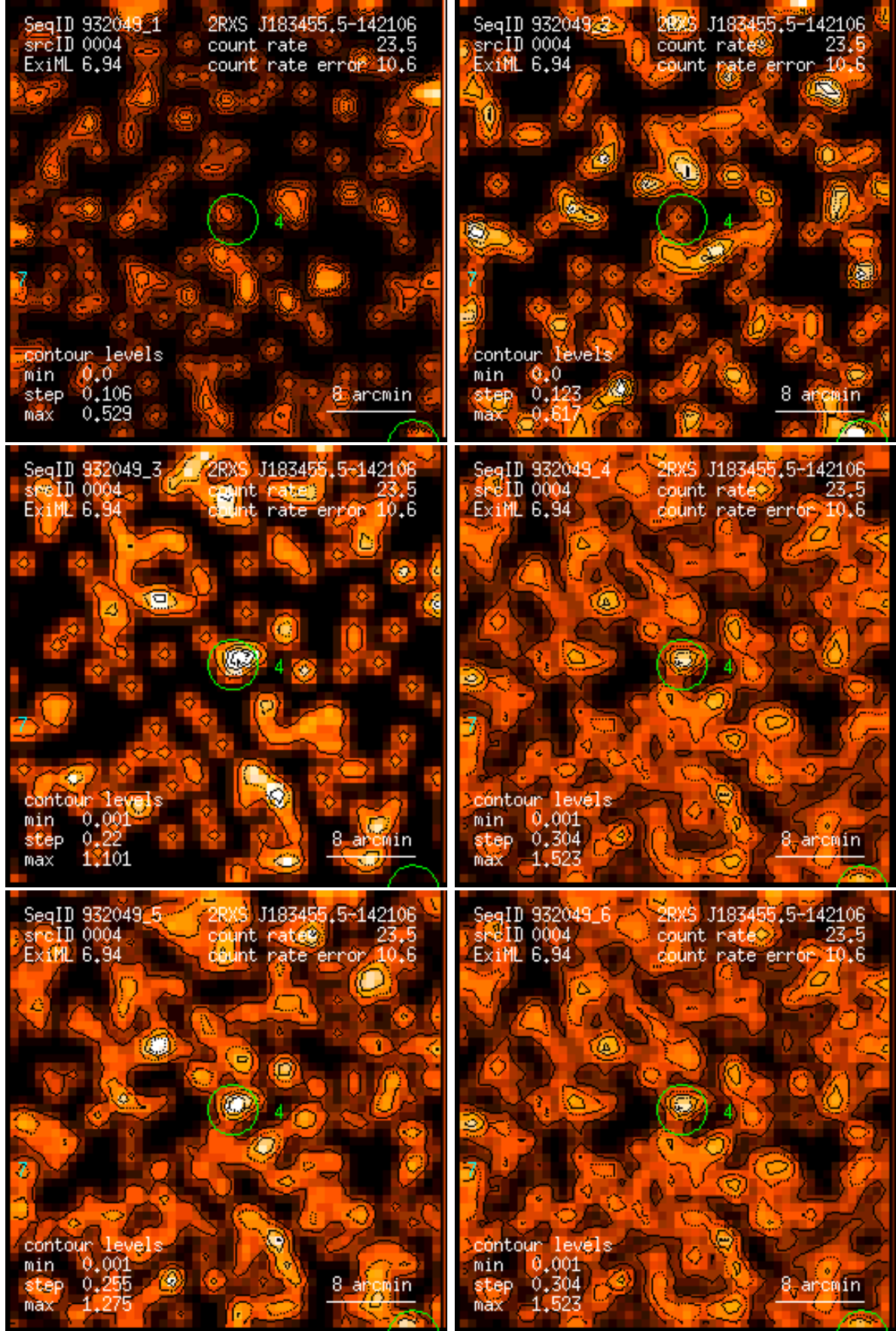
Figure 4: RASS 932049: detection 0004: band rate images, Gaussian filter: (1) PSPC channels 11 – 41, (2) 52 – 90, (3) 91 – 201, (4) 11 – 235, (5) 52 – 201, (6) 11 – 201. Broad band rates in counts/ks. Band rate contour levels in counts/ks/arcmin 2 .
