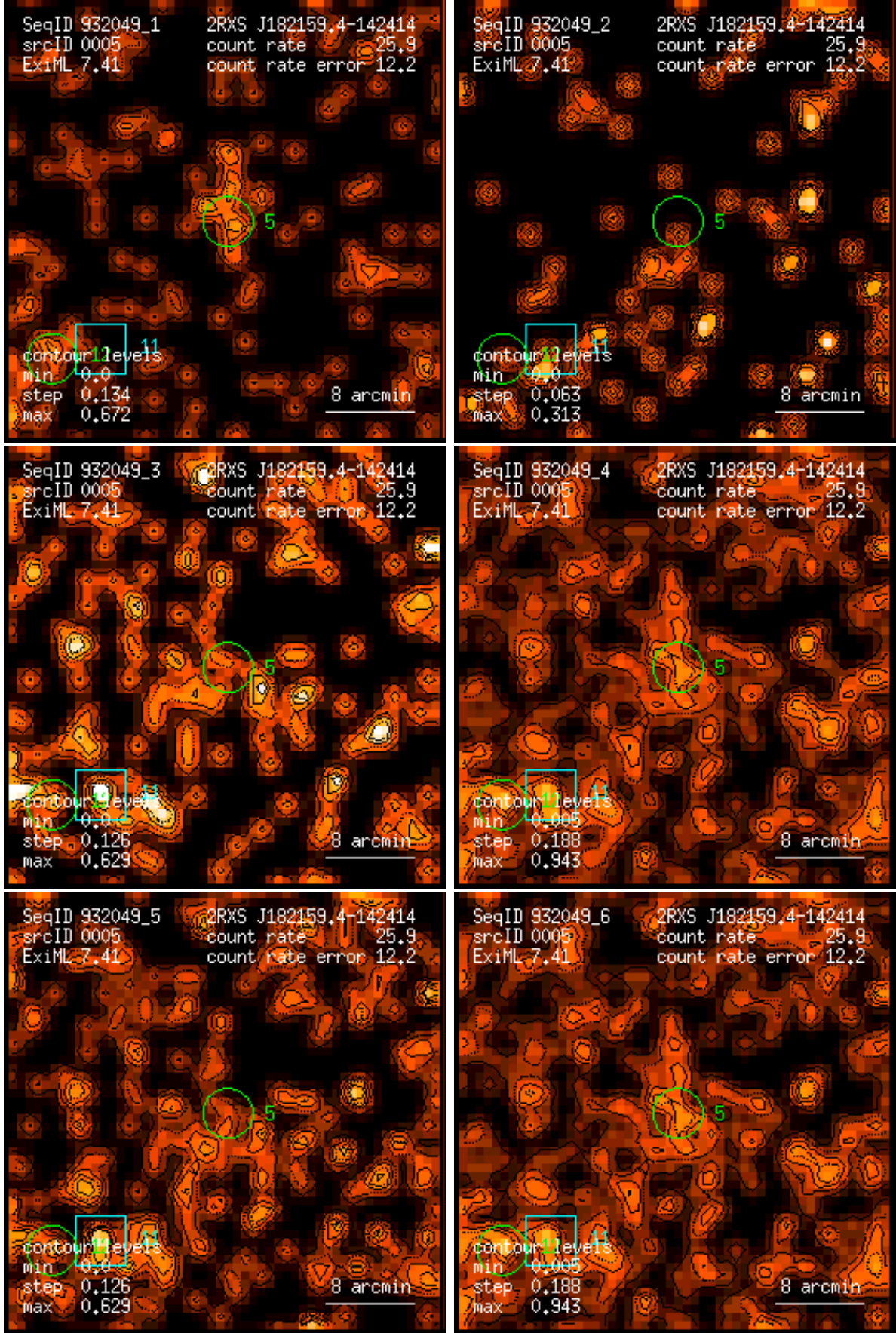
Figure 5: RASS 932049: detection 0005: band rate images, Gaussian filter: (1) PSPC channels 11 – 41, (2) 52 – 90, (3) 91 – 201, (4) 11 – 235, (5) 52 – 201, (6) 11 – 201. Broad band rates in counts/ks. Band rate contour levels in counts/ks/arcmin 2 .
