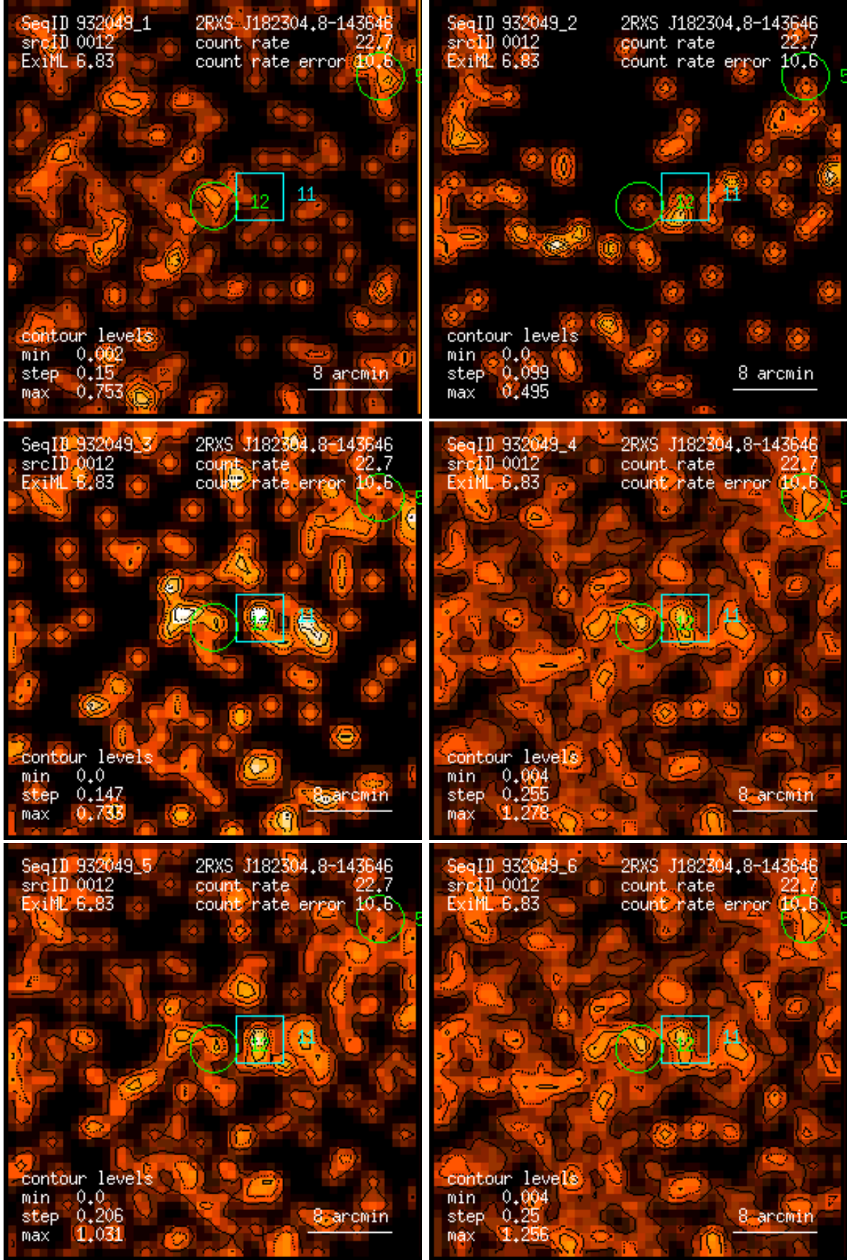
Figure 12: RASS 932049: detection 0012: band rate images, Gaussian filter: (1) PSPC channels 11 – 41, (2) 52 – 90, (3) 91 – 201, (4) 11 – 235, (5) 52 – 201, (6) 11 – 201. Broad band rates in counts/ks. Band rate contour levels in counts/ks/arcmin 2 .
