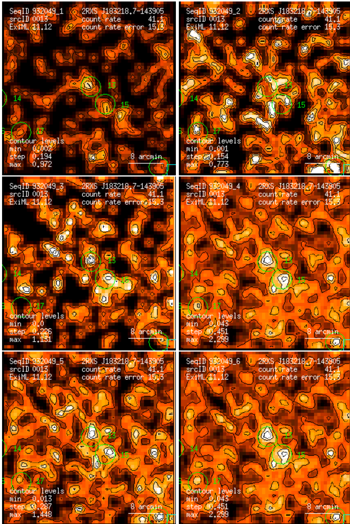
Figure 13: RASS 932049: detection 0013: band rate images, Gaussian filter: (1) PSPC channels 11 – 41, (2) 52 – 90, (3) 91 – 201, (4) 11 – 235, (5) 52 – 201, (6) 11 – 201. Broad band rates in counts/ks. Band rate contour levels in counts/ks/arcmin 2 .
