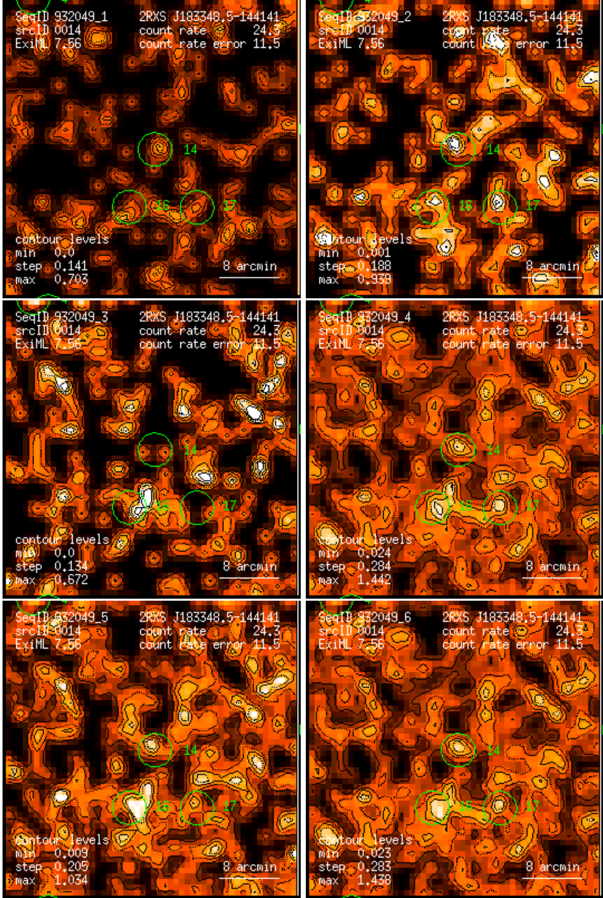
Figure 14: RASS 932049: detection 0014: band rate images, Gaussian filter: (1) PSPC channels 11 – 41, (2) 52 – 90, (3) 91 – 201, (4) 11 – 235, (5) 52 – 201, (6) 11 – 201. Broad band rates in counts/ks. Band rate contour levels in counts/ks/arcmin 2 .
