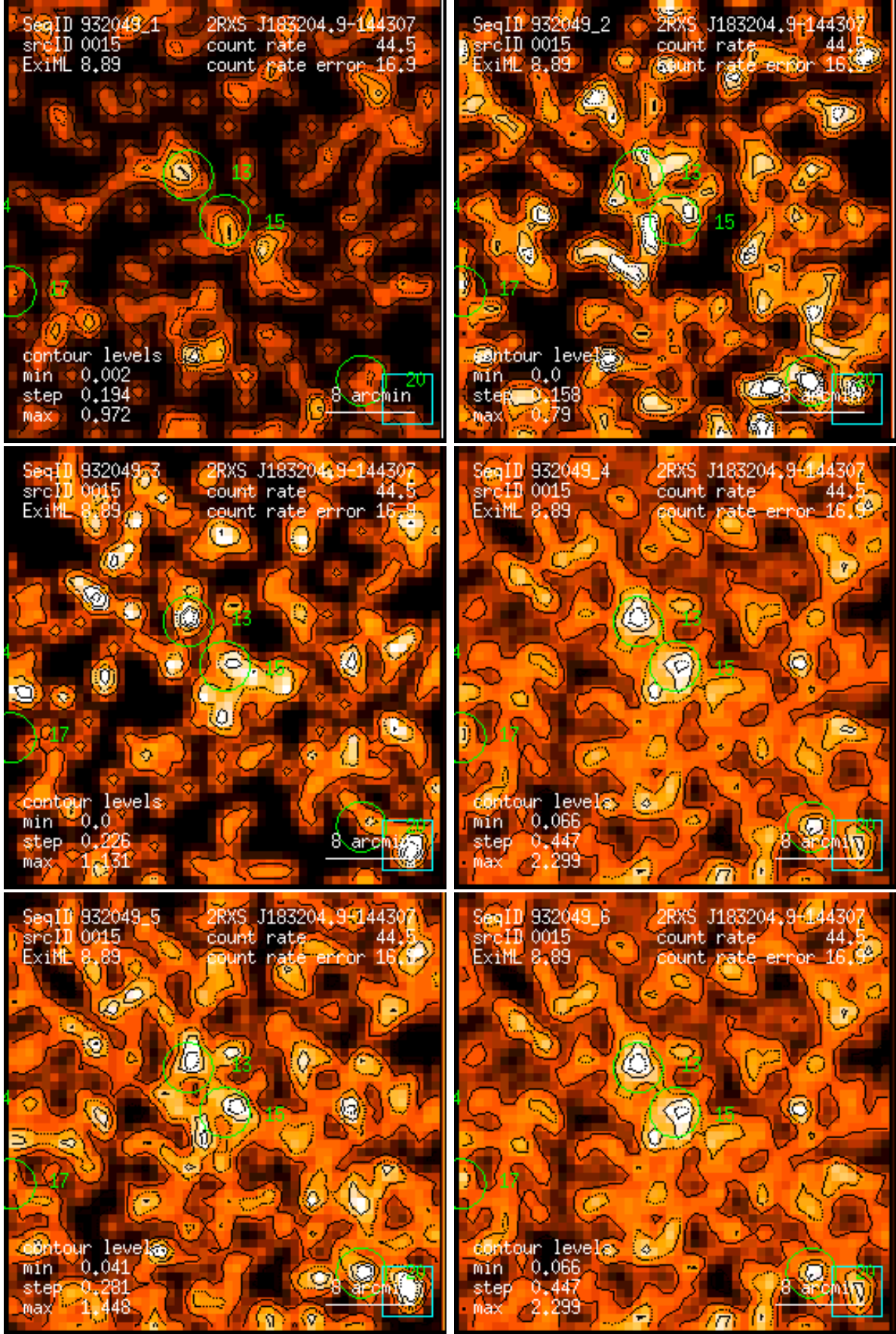
Figure 15: RASS 932049: detection 0015: band rate images, Gaussian filter: (1) PSPC channels 11 – 41, (2) 52 – 90, (3) 91 – 201, (4) 11 – 235, (5) 52 – 201, (6) 11 – 201. Broad band rates in counts/ks. Band rate contour levels in counts/ks/arcmin 2 .
