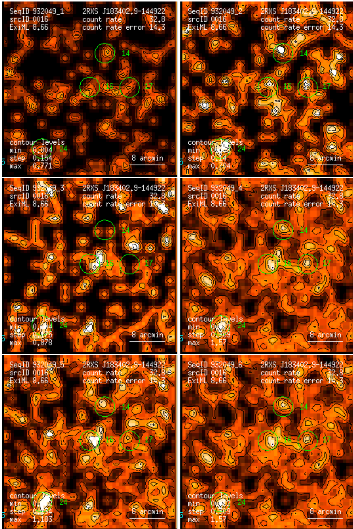
Figure 16: RASS 932049: detection 0016: band rate images, Gaussian filter: (1) PSPC channels 11 – 41, (2) 52 – 90, (3) 91 – 201, (4) 11 – 235, (5) 52 – 201, (6) 11 – 201. Broad band rates in counts/ks. Band rate contour levels in counts/ks/arcmin 2 .
