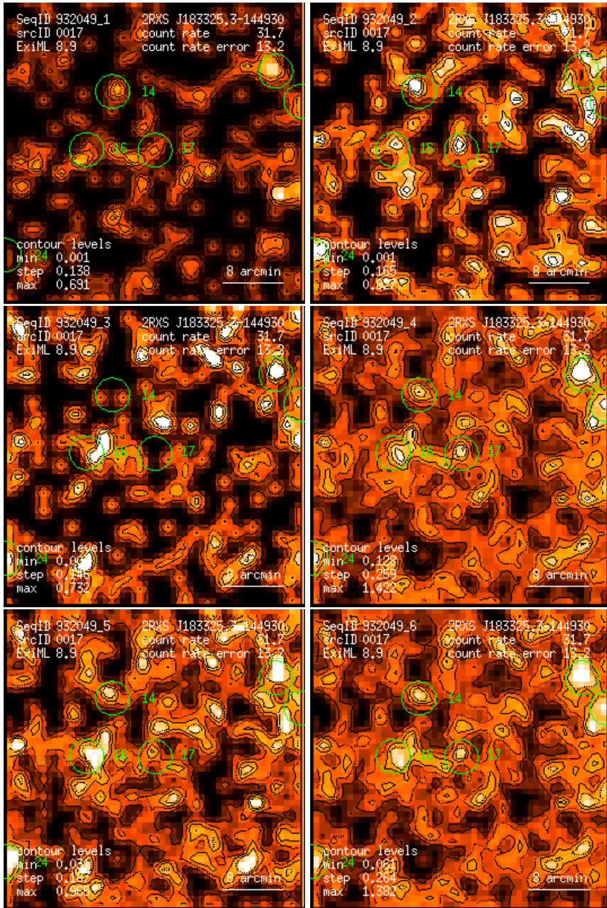
Figure 17: RASS 932049: detection 0017: band rate images, Gaussian filter: (1) PSPC channels 11 – 41, (2) 52 – 90, (3) 91 – 201, (4) 11 – 235, (5) 52 – 201, (6) 11 – 201. Broad band rates in counts/ks. Band rate contour levels in counts/ks/arcmin 2 .
