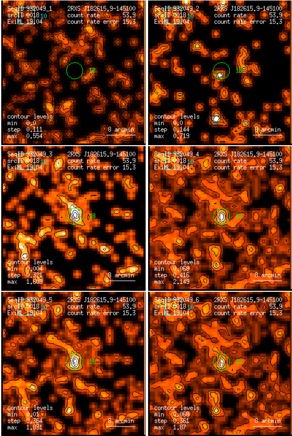
Figure 18: RASS 932049: detection 0018: band rate images, Gaussian filter: (1) PSPC channels 11 – 41, (2) 52 – 90, (3) 91 – 201, (4) 11 – 235, (5) 52 – 201, (6) 11 – 201. Broad band rates in counts/ks. Band rate contour levels in counts/ks/arcmin 2 .
