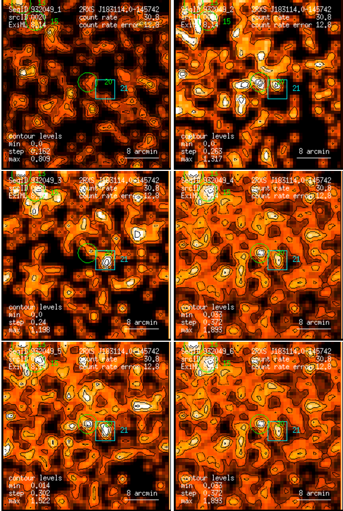
Figure 20: RASS 932049: detection 0020: band rate images, Gaussian filter: (1) PSPC channels 11 – 41, (2) 52 – 90, (3) 91 – 201, (4) 11 – 235, (5) 52 – 201, (6) 11 – 201. Broad band rates in counts/ks. Band rate contour levels in counts/ks/arcmin 2 .
