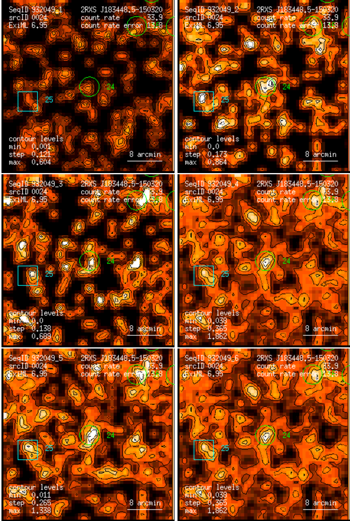
Figure 24: RASS 932049: detection 0024: band rate images, Gaussian filter: (1) PSPC channels 11 – 41, (2) 52 – 90, (3) 91 – 201, (4) 11 – 235, (5) 52 – 201, (6) 11 – 201. Broad band rates in counts/ks. Band rate contour levels in counts/ks/arcmin 2 .
