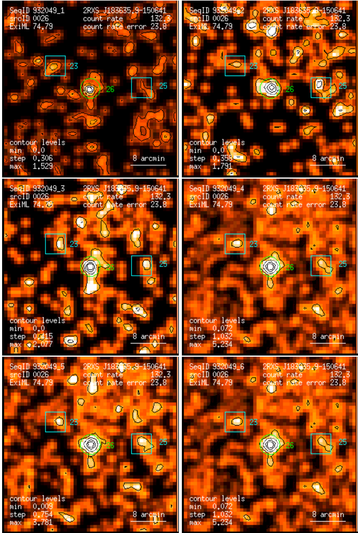
Figure 26: RASS 932049: detection 0026: band rate images, Gaussian filter: (1) PSPC channels 11 – 41, (2) 52 – 90, (3) 91 – 201, (4) 11 – 235, (5) 52 – 201, (6) 11 – 201. Broad band rates in counts/ks. Band rate contour levels in counts/ks/arcmin 2 .
