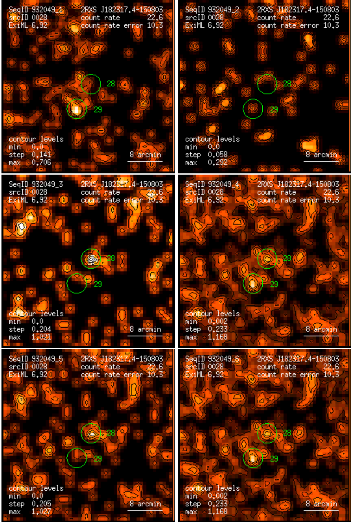
Figure 28: RASS 932049: detection 0028: band rate images, Gaussian filter: (1) PSPC channels 11 – 41, (2) 52 – 90, (3) 91 – 201, (4) 11 – 235, (5) 52 – 201, (6) 11 – 201. Broad band rates in counts/ks. Band rate contour levels in counts/ks/arcmin 2 .
