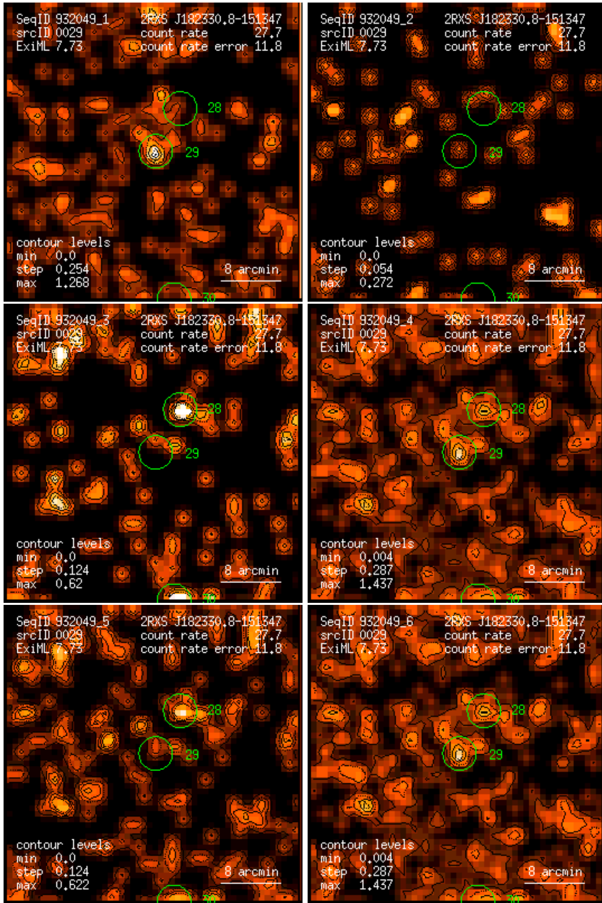
Figure 29: RASS 932049: detection 0029: band rate images, Gaussian filter: (1) PSPC channels 11 – 41, (2) 52 – 90, (3) 91 – 201, (4) 11 – 235, (5) 52 – 201, (6) 11 – 201. Broad band rates in counts/ks. Band rate contour levels in counts/ks/arcmin 2 .
