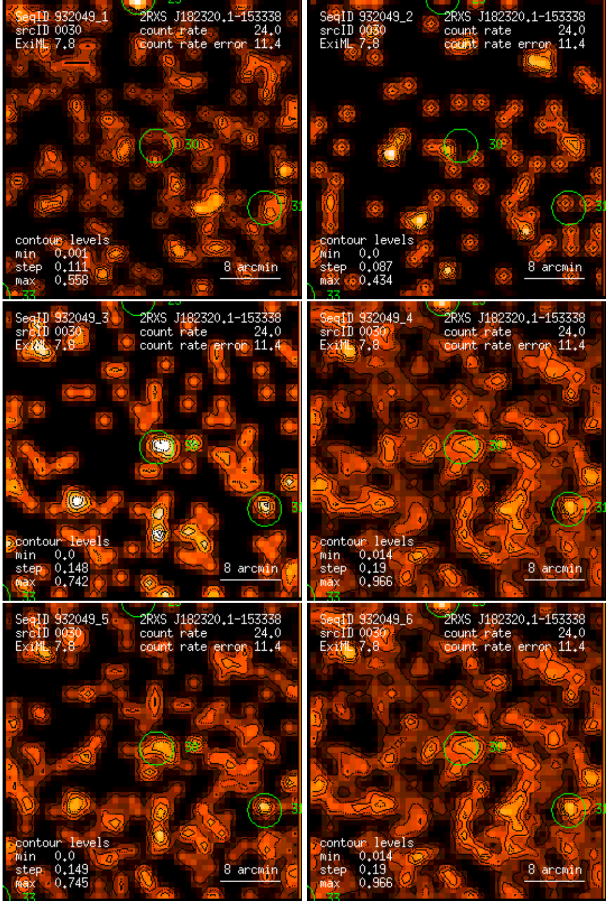
Figure 30: RASS 932049: detection 0030: band rate images, Gaussian filter: (1) PSPC channels 11 – 41, (2) 52 – 90, (3) 91 – 201, (4) 11 – 235, (5) 52 – 201, (6) 11 – 201. Broad band rates in counts/ks. Band rate contour levels in counts/ks/arcmin 2 .
