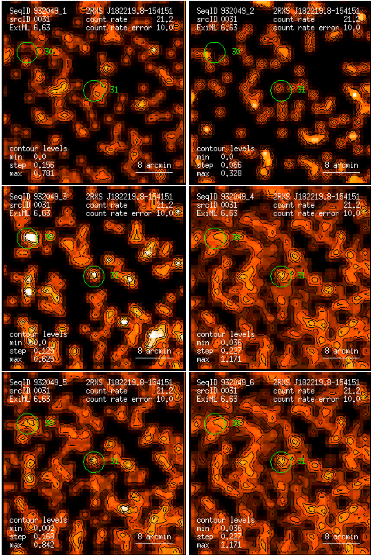
Figure 31: RASS 932049: detection 0031: band rate images, Gaussian filter: (1) PSPC channels 11 – 41, (2) 52 – 90, (3) 91 – 201, (4) 11 – 235, (5) 52 – 201, (6) 11 – 201. Broad band rates in counts/ks. Band rate contour levels in counts/ks/arcmin 2 .
