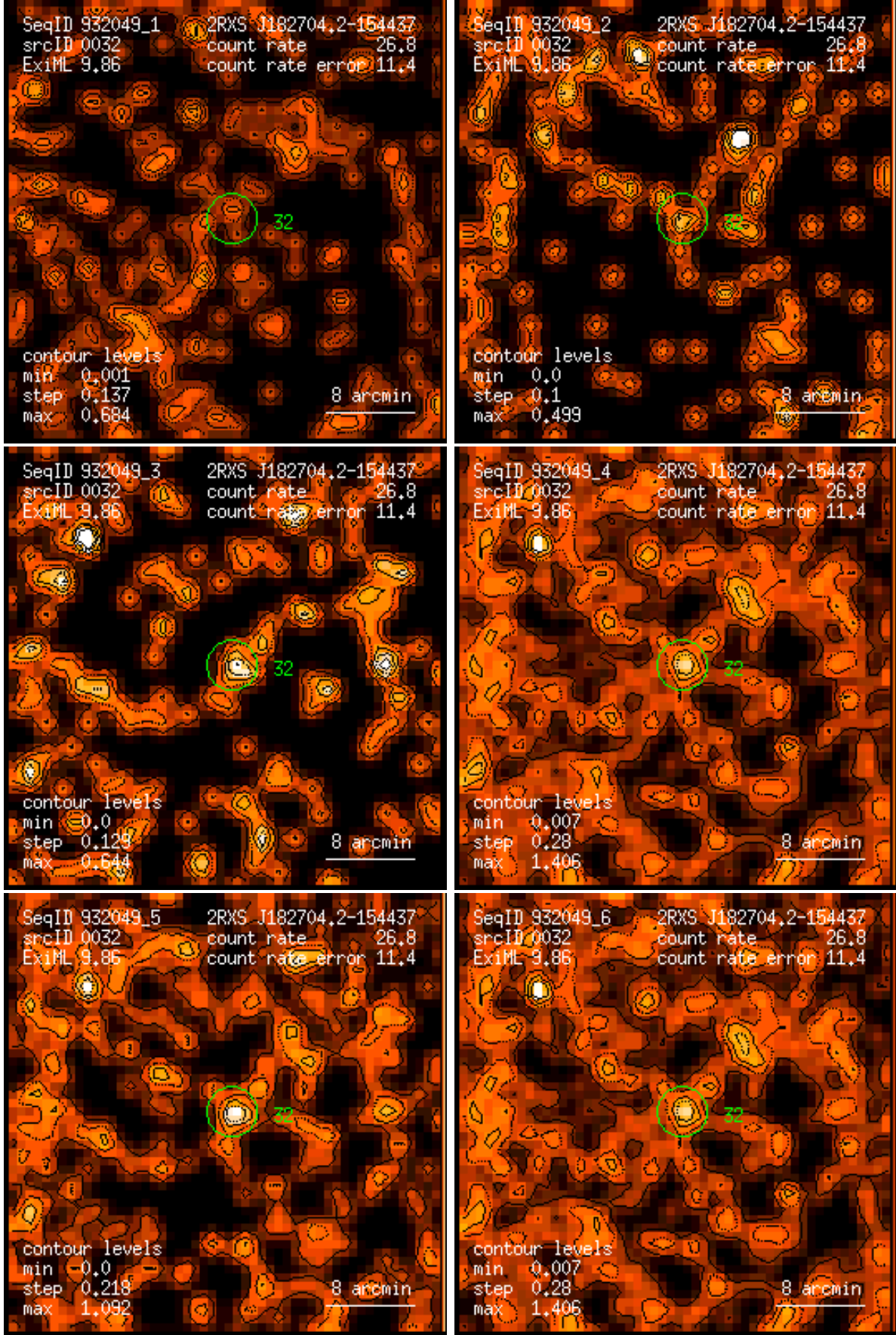
Figure 32: RASS 932049: detection 0032: band rate images, Gaussian filter: (1) PSPC channels 11 – 41, (2) 52 – 90, (3) 91 – 201, (4) 11 – 235, (5) 52 – 201, (6) 11 – 201. Broad band rates in counts/ks. Band rate contour levels in counts/ks/arcmin 2 .
