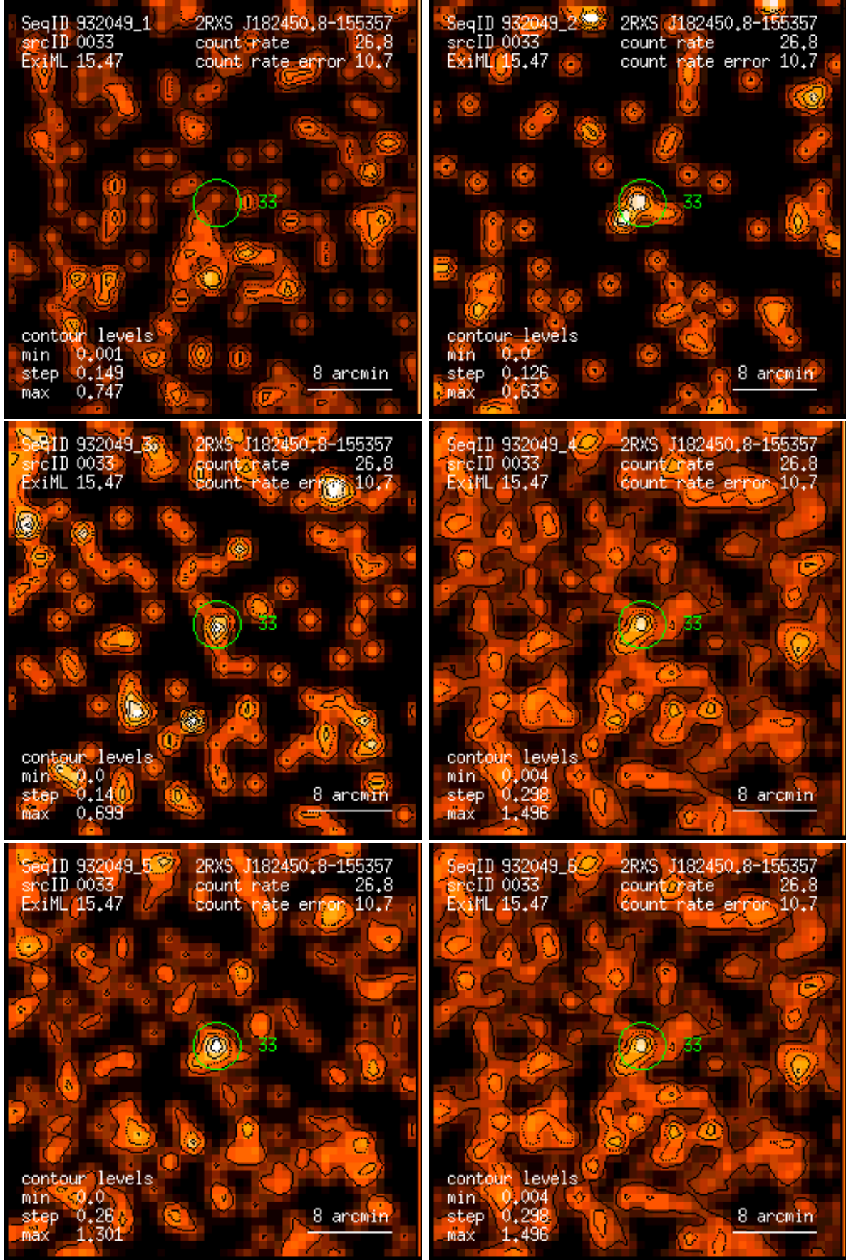
Figure 33: RASS 932049: detection 0033: band rate images, Gaussian filter: (1) PSPC channels 11 – 41, (2) 52 – 90, (3) 91 – 201, (4) 11 – 235, (5) 52 – 201, (6) 11 – 201. Broad band rates in counts/ks. Band rate contour levels in counts/ks/arcmin 2 .
