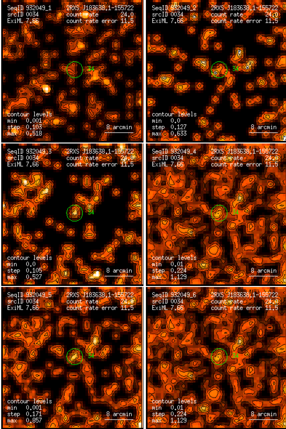
Figure 34: RASS 932049: detection 0034: band rate images, Gaussian filter: (1) PSPC channels 11 – 41, (2) 52 – 90, (3) 91 – 201, (4) 11 – 235, (5) 52 – 201, (6) 11 – 201. Broad band rates in counts/ks. Band rate contour levels in counts/ks/arcmin 2 .
