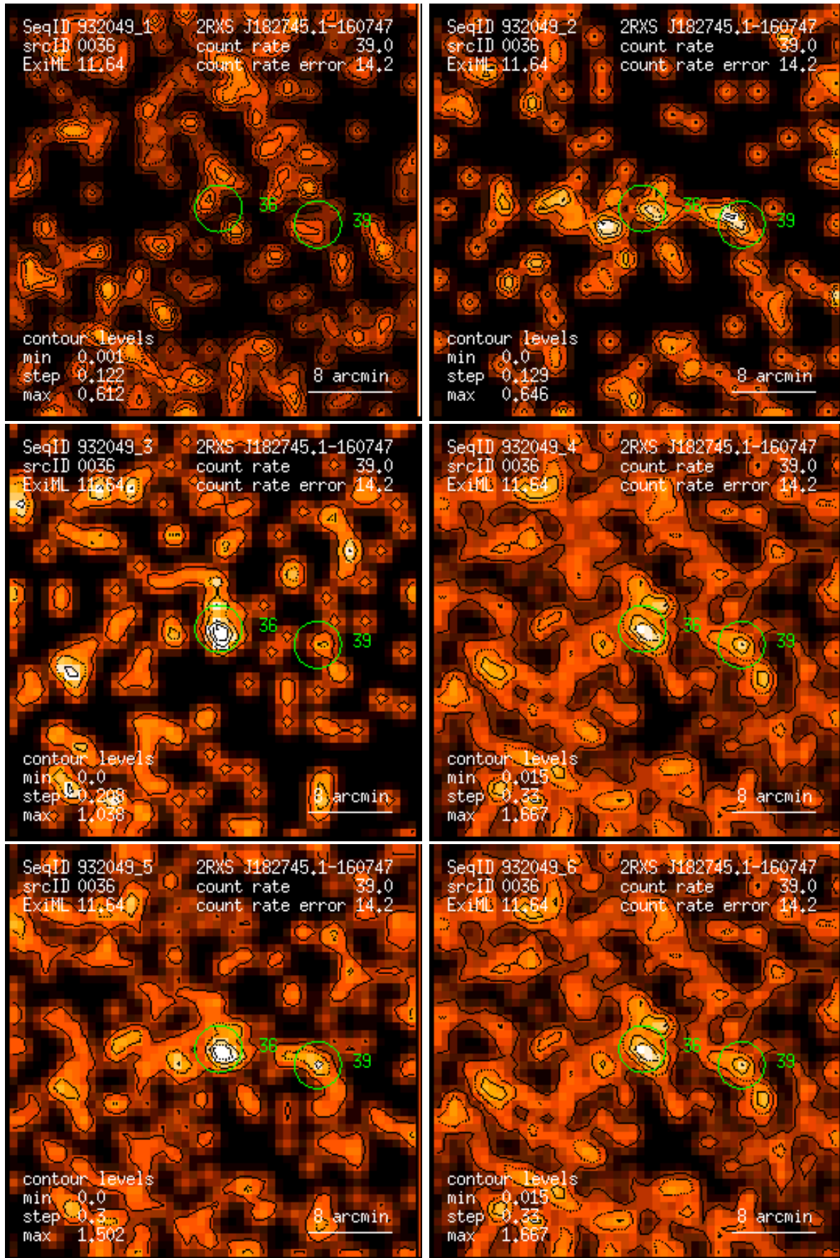
Figure 36: RASS 932049: detection 0036: band rate images, Gaussian filter: (1) PSPC channels 11 – 41, (2) 52 – 90, (3) 91 – 201, (4) 11 – 235, (5) 52 – 201, (6) 11 – 201. Broad band rates in counts/ks. Band rate contour levels in counts/ks/arcmin 2 .
