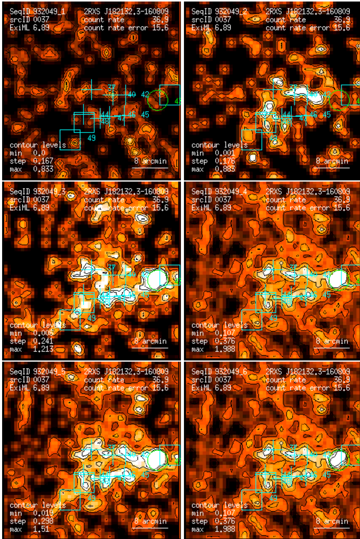
Figure 37: RASS 932049: detection 0037: band rate images, Gaussian filter: (1) PSPC channels 11 – 41, (2) 52 – 90, (3) 91 – 201, (4) 11 – 235, (5) 52 – 201, (6) 11 – 201. Broad band rates in counts/ks. Band rate contour levels in counts/ks/arcmin 2 .
