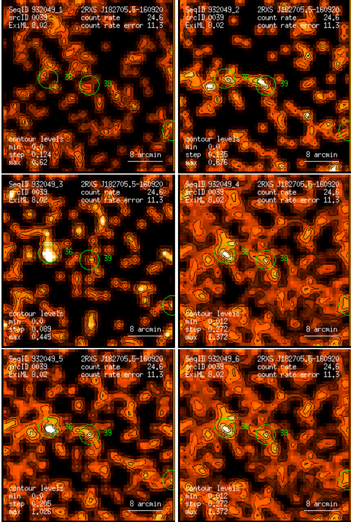
Figure 39: RASS 932049: detection 0039: band rate images, Gaussian filter: (1) PSPC channels 11 – 41, (2) 52 – 90, (3) 91 – 201, (4) 11 – 235, (5) 52 – 201, (6) 11 – 201. Broad band rates in counts/ks. Band rate contour levels in counts/ks/arcmin 2 .
