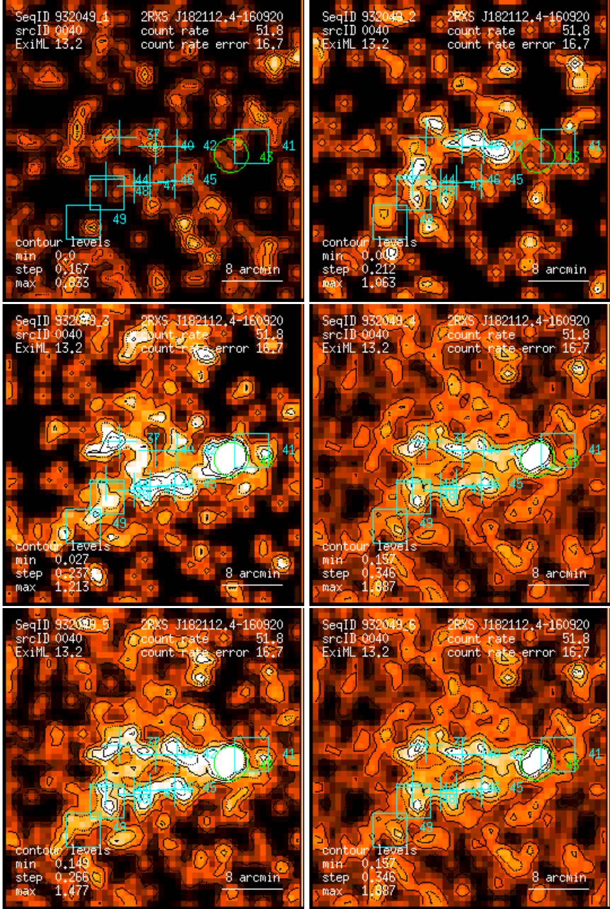
Figure 40: RASS 932049: detection 0040: band rate images, Gaussian filter: (1) PSPC channels 11 – 41, (2) 52 – 90, (3) 91 – 201, (4) 11 – 235, (5) 52 – 201, (6) 11 – 201. Broad band rates in counts/ks. Band rate contour levels in counts/ks/arcmin 2 .
